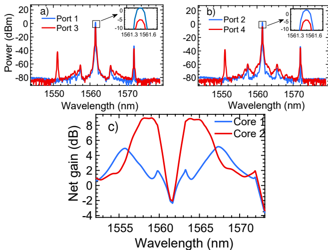
Fig. 5. Power and gain spectrum of core 1 and 2. Input (blue) and output (red) power spectrum of a) core 1 and b) core 2. Gain spectrum of both cores in c). Insets in a) and b) details input and output power losses. In a) and b) signal wave is placed at 1572 nm.
