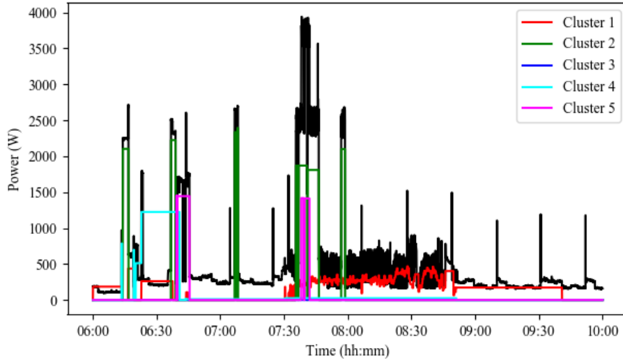
435 436 Figure 12. Reconstructed power profile of individual states learnt from the data and the aggregate consumption.
