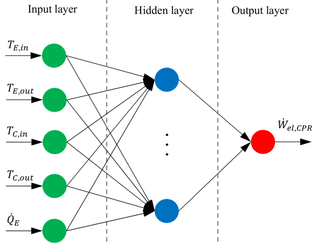
Figure 4: Topology of the applied feed-forward neural network with the corresponding input and output variables.
