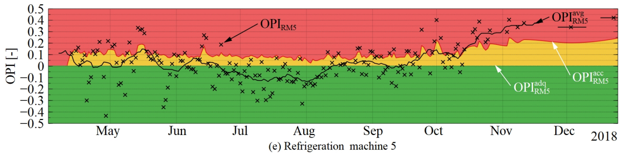
Figure 6: Optimization potential index OPI_{RM} of (a) refrigeration machine 1 to (e) refrigeration machine 5 with adequate (green), acceptable (yellow) and inadequate (red) operation range. The data points (black crosses) represent the daily OPI values and the black solid line indicates the 14-days moving average of the OPI.
