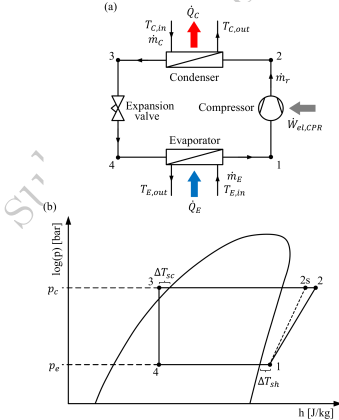
Figure 3: Simplified schematic of (a) the considered refrigeration cycle and (b) the corresponding log(p)-h-diagram with the different refrigerant states 1 to 4 and 2s.
