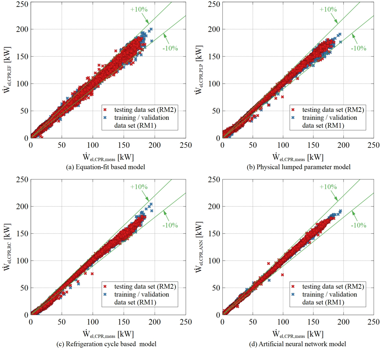
Figure 5: Comparison of the measured and modeled compressor electrical power consumption of the refrigeration machines in the field plant: (a) equation-fit based model, (b) physical lumped parameter model, (c) refrigeration cycle based model and (d) artificial neural network model.
