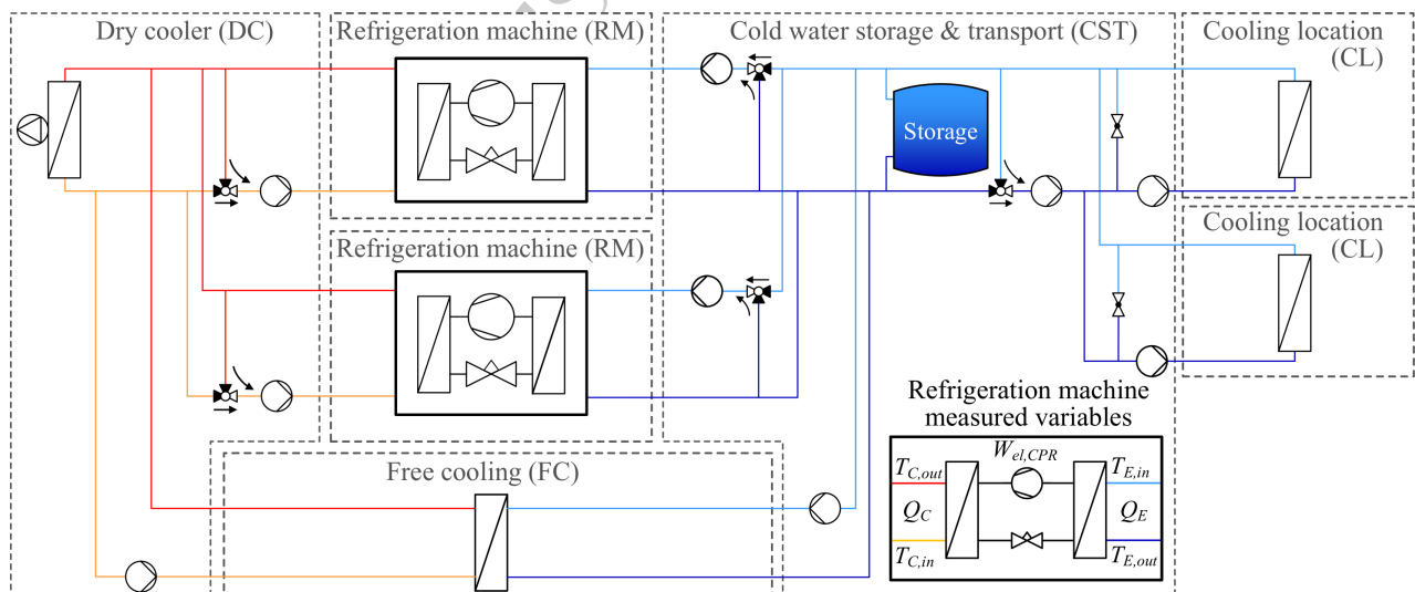
Figure 2: Simplified piping & instrumentation diagram of a typical refrigeration plant with cold water distribution and a free cooling module, i.e. heat exchanger. Commonly measured and monitored variables of refrigeration machines in field plants are shown in italic.
