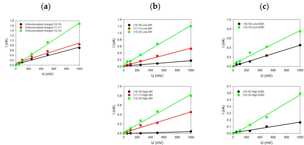
Figure 3. (a) Theoretical curves I = f(V) for different charged SWCNT with ends (a) unfunctionalized; (b) functionalized with -OH (top: low functionalization rate; bottom: high functionalization rate); (c) functionalized with -COO^- (top: low functionalization rate; bottom: high functionalization rate).
