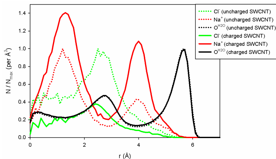
Figure 6. Water and ion distribution per elementary volume inside (13,13) CNT ( \text{Cl}^- ions are in green lines; \text{Na}^+ in red and water in black lines). Results have been obtained for uncharged (dotted) and charged carbon atoms (full lines), respectively. The ion distributions were normalized according to the maximum value of each distribution in the uncharged case, in order to compare the uncharged and charged SWCNT correctly.
