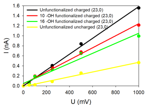
Figure 5. Theoretical curves I = f(V) for different (23,0) SWCNT.
