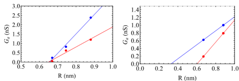
Figure 4. Access conductance G_a (in nS) as a function of the SWCNT radius R (in nm) with ends functionalized with -OH (left) and -COO^- (right) at low functionalization degree (blue) and high functionalization one (red). The lines correspond to linear fits (values given in the text).
