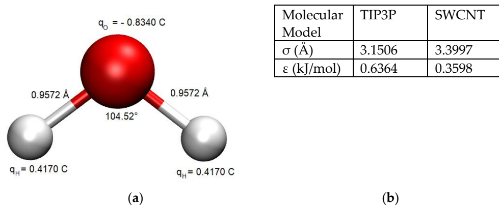
Figure 2. (a) Representation of TIP3P. Oxygen and Hydrogen atoms are shown in red and in white, respectively. (b) Van der Waals parameters for water model and SWCNT atoms.
