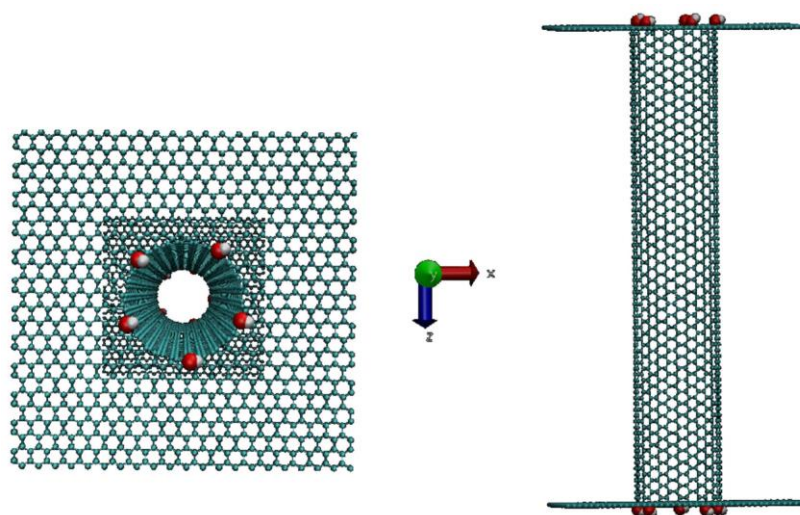
Figure 1. System (10,10) SWCNT functionalized by -\text{OH} functions. Top view ( left ) and side view ( right ) before optimization.
