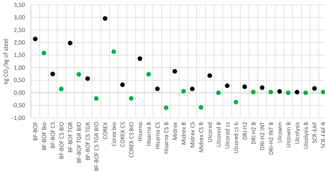
Figure 4: Maximum CO 2 emissions by steel producing technology represented in the TIAM-FR model.
