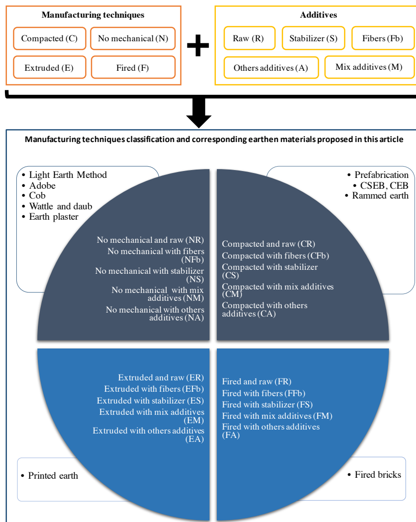
Figure 6. Excavated soil valorization techniques classification.
