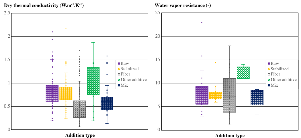
Figure 9. Effects of additives on hygrothermal properties.
