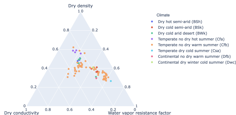
Figure 19. MATARUN Diagram N°2: ternary diagram of relationship between hygrothermal and physical properties balances and study climate zones.
