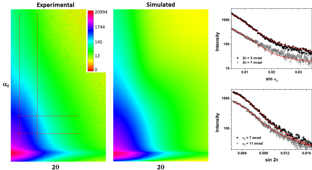
FIG. 2. (Color online) Experimental GISAXS pattern (left), compared to simulated one (middle), with the 4 sections (right: experimental dots and simulated lines) used to find the best fit parameters (given in text). The 4 sections used are shown as vertical and horizontal lines on the experimental GISAXS pattern.
