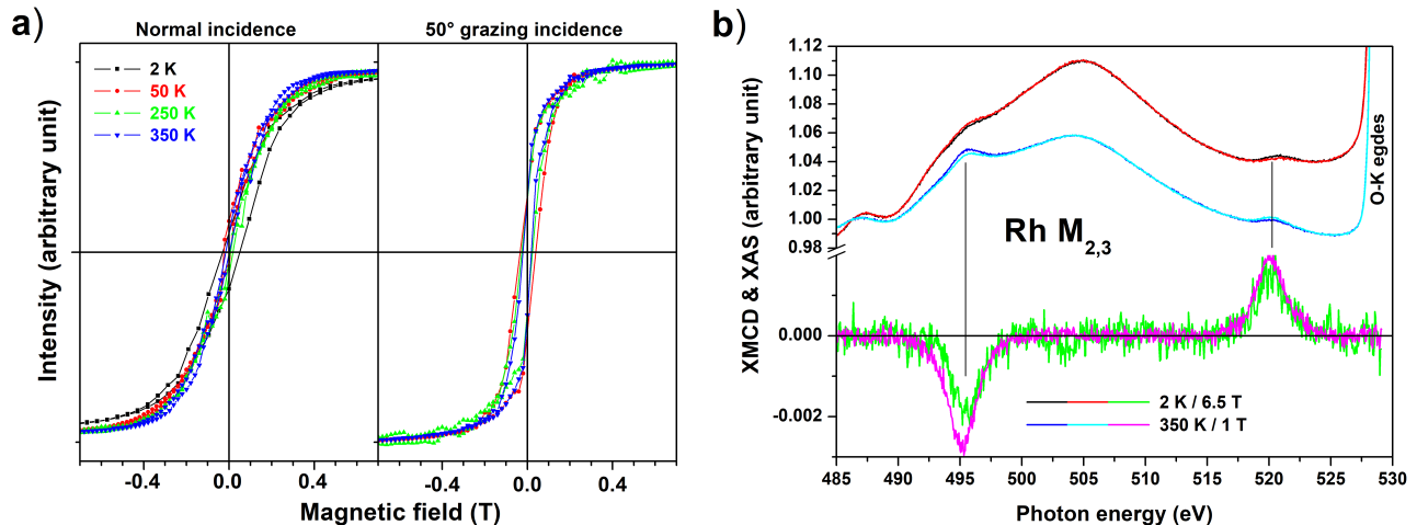
FIG. 7. (Color online) XMCD measurements on the FeRh particles of Section IV. a) Hysteresis loops measured at the Fe L 3 edge (maximum XMCD signal), for different temperatures, with a normal or grazing incidence of the x-ray beam (and thus a different direction of the applied magnetic field). b) XAS and XMCD signals at the Rh M 2,3 edges, at 350 K and 2 K for a normal incidence.
