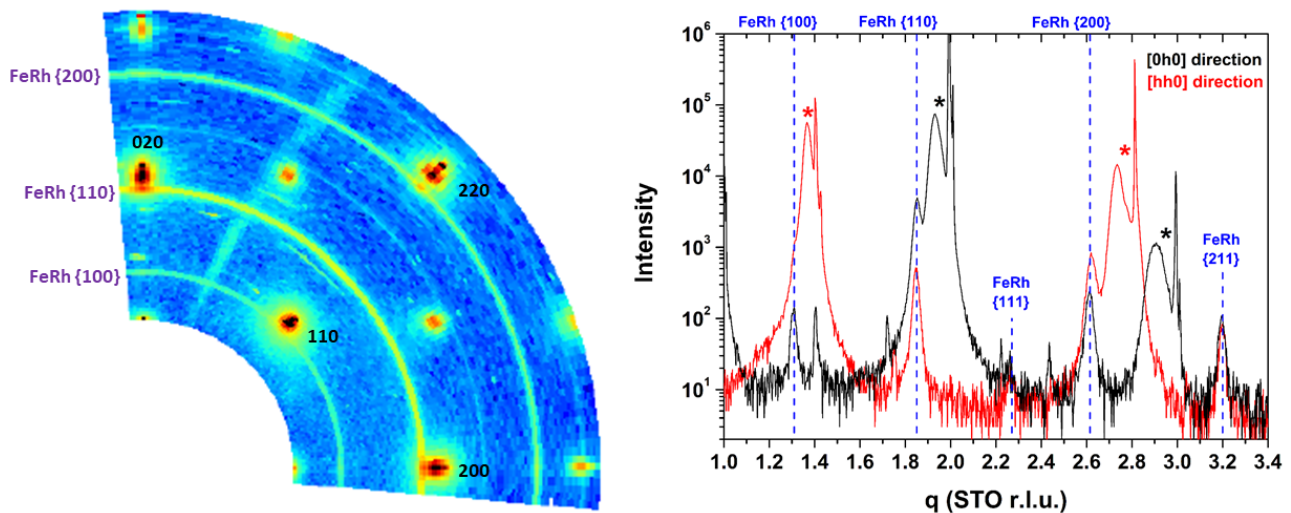
FIG. 5. (Color online) Left: reciprocal space map measured by GIXRD (the color correspond to log scale of the intensity) in a h, k projection ( l \simeq 0 ). The main peaks correspond to the substrate (integer value of h, k ). FeRh peaks are detected as rings, with higher intensity in particular azimuths. Right: GIXRD radial scan in particular directions in the surface plane. Some small parasitic peaks are also visible in addition to the FeRh “ring” signal and to the most intense diffraction peaks of the substrate, marked with a star (STO crystal and relaxed BTO thin film, appearing as a shoulder on the low- q side).
