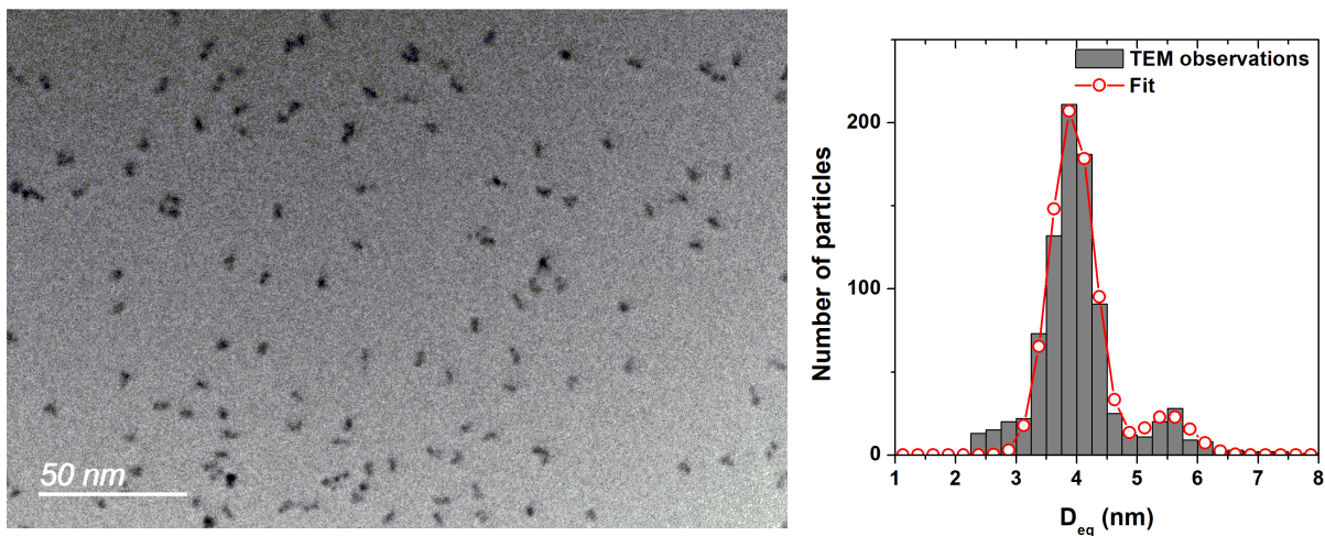
FIG. 1. (Color online) Left: TEM image of the incident FeRh clusters, deposited here on an amorphous carbon layer. Right: size histogram deduced from TEM observations, with a fit using two Gaussians (for the main monomer peak and the small dimer peak).
