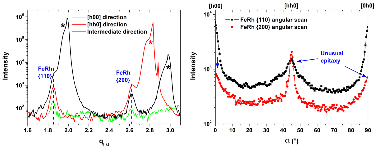
FIG. 3. (Color online) Left: GIXRD measurements (radial scans in the reciprocal space, at constant l \simeq 0 , and with the wavevector expressed in STO relative lattice unit), in logarithmic intensity scale, along different in-plane directions ( [h00] , [hh0] of BTO and intermediate direction in between). \{110\}_{\text{FeRh}} and \{200\}_{\text{FeRh}} peaks are visible in addition to substrate peaks marked with stars (STO crystal and BTO thin film, appearing as a shoulder on the left side). Right: Angular scan, i.e. along different in-plane directions, for the wavevector q corresponding to \{110\}_{\text{FeRh}} and \{200\}_{\text{FeRh}} peaks. The unusual epitaxy results in a higher intensity in particular azimuths of the BTO crystal.
