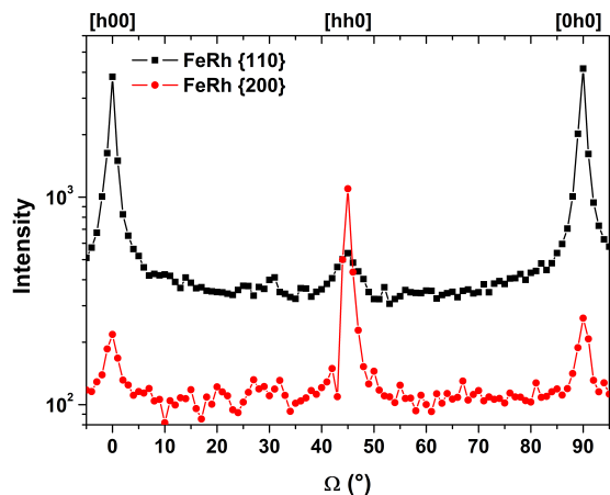
FIG. 6. (Color online) Intensity of \{110\}_{\text{FeRh}} and \{200\}_{\text{FeRh}} peaks deduced from angular scans, i.e. along different in-plane directions. The background signal coming from the substrate peaks has been subtracted when needed. The higher intensity along particular directions is the signature of preferential orientations (epitaxy relationships).
