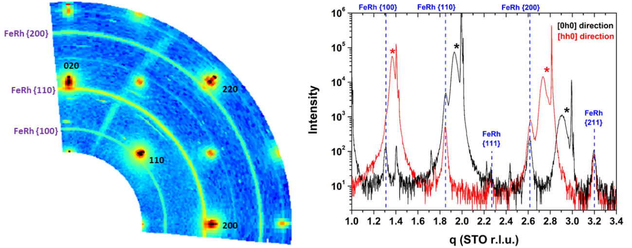
FIG. 5. (Color online) Left: reciprocal space map measured by GIXRD (the color correspond to log scale of the intensity) in a h, k projection ( l \simeq 0 ). The main peaks correspond to the substrate (integer value of h, k ). FeRh peaks are detected as rings, with higher intensity in particular azimuths. Right: GIXRD radial scan in particular directions in the surface plane. Some small parasitic peaks are also visible in addition to the FeRh “ring” signal and to the most intense diffraction peaks of the substrate, marked with a star (STO crystal and relaxed BTO thin film, appearing as a shoulder on the low- q side).
