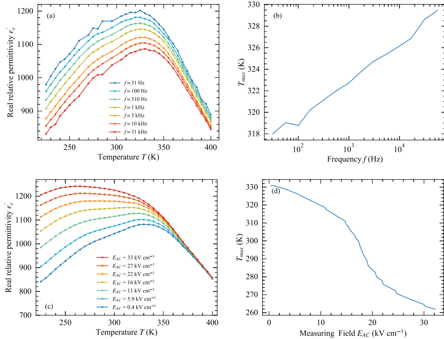
Figure 2. Relative permittivity as a function of the temperature for different measurement frequency for E_{AC} = 1.2 \text{ kV cm}^{-1} (a). T_{max} for which the relative permittivity is maximum as a function of the frequency for E_{AC} = 1.2 \text{ kV cm}^{-1} (b). Relative permittivity as a function of the temperature for different values of the AC measuring field for f = 10 \text{ kHz} (c). T_{max} for which the relative permittivity is maximum as a function of the AC measuring field for f = 10 \text{ kHz} (d).
