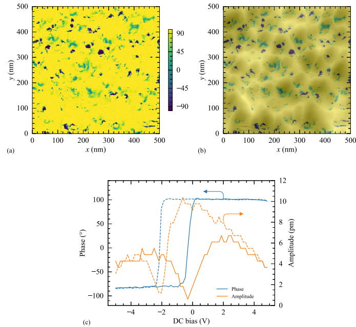
Figure 1. Phase of the Vertical PFM (VPPM) (a). Superimposition of the phase signal and the topography (b). PFM phase and amplitude as a function of an applied DC voltage V_{DC} (c).
