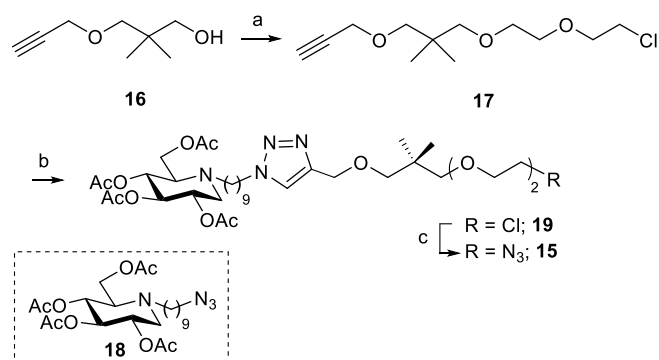
Scheme 1. Reagents and conditions: Synthesis of DNJ-linker conjugate 15 : (a) 1-Chloro-2-(2-chloroethoxy)ethane, 50% aq. NaOH, n -Bu 4 NHSO 4 , 35 °C (62%); (b) 18 , CuSO 4 ·5H 2 O cat., sodium ascorbate, DMF/H 2 O, MW, 80 °C (98%); (c) n -Bu 4 NI, NaN 3 , DMF, 80 °C (95%).
