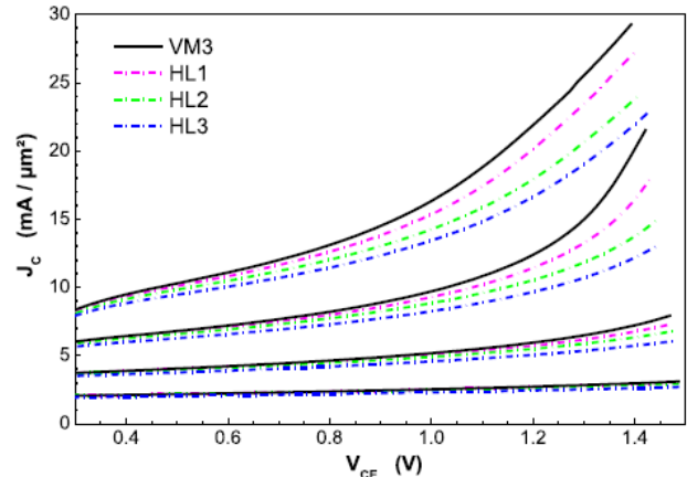
Fig. 9: Collector current density J_C for the test structures. The V_{BE} is swept from 0.825 to 0.9 \text{ V} . [Esp16]
