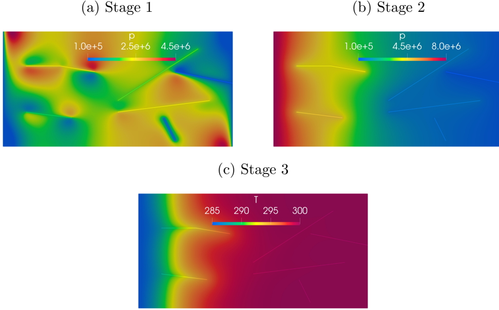
Figure 8. Discrete solution obtained with the enthalpy-based model on the finest mesh m = 3 : (a) pressure p at the very beginning of stage 1 ( t = 0.1 s), (b) pressure p at t = 116 s during stage 2, (c) temperature T at t = 27715 s time during stage 3.
