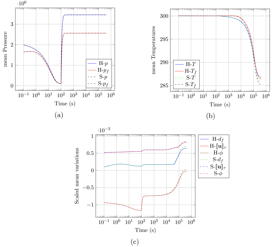
Figure 10. (a) Matrix and fracture mean pressures, (b) matrix and fracture mean temperatures, and (c) scaled mean \llbracket \mathbf{u} \rrbracket_\tau , d_f - d_0 and \phi - \phi^0 as functions of time for the solutions on the finest mesh m = 3 , for the discretisations of the enthalpy-based (H) and entropy-based (S) models.
