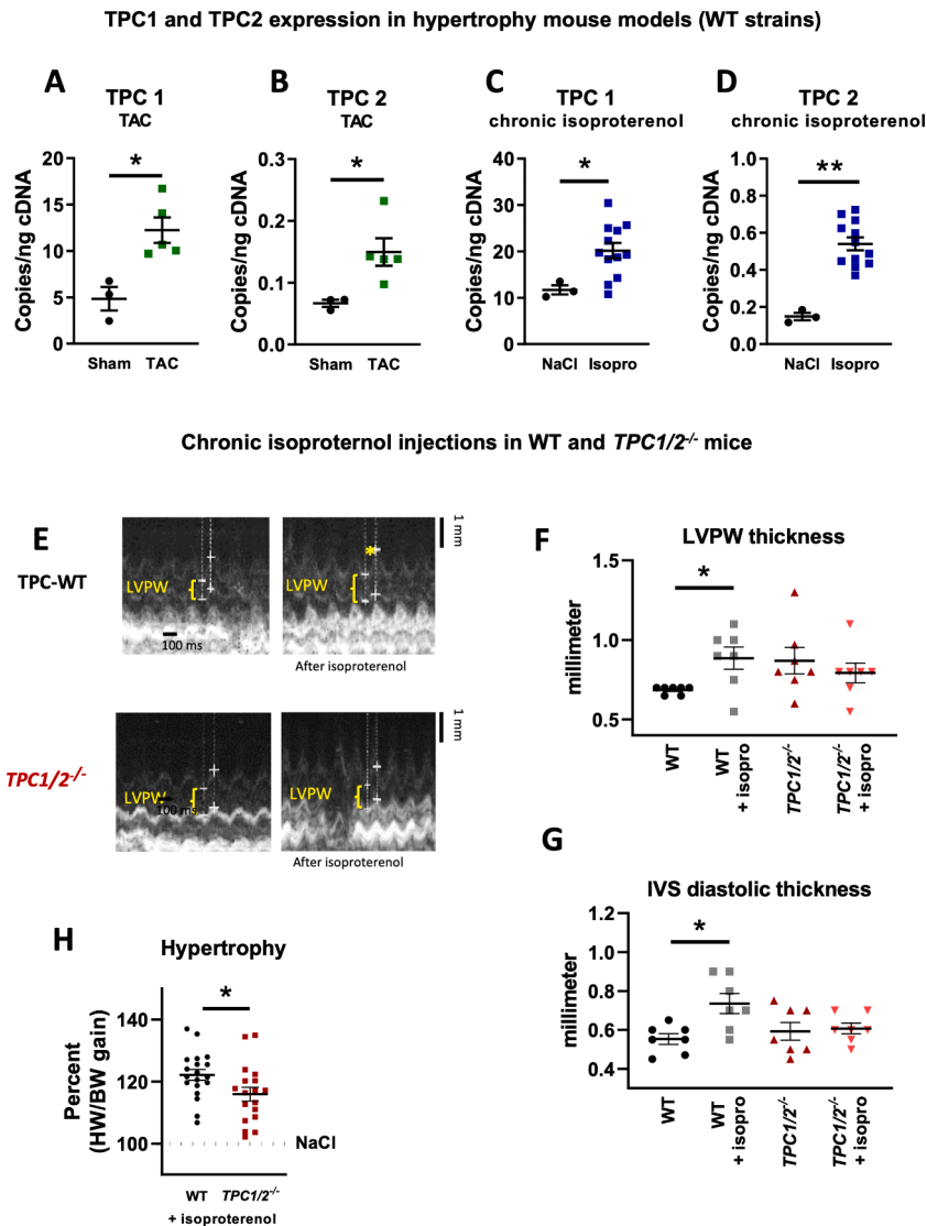
Fig. 5. TPCs are highly expressed in hypertrophic heart and their deletion reduced the heart hypertrophy induced by chronic isoproterenol injections. (A, B) Quantification by RT-qPCR of the absolute levels of Tpcn1 and Tpcn2 transcripts in sham mice hearts and after a TAC surgery ( N = 3 Sham mice; N = 5 TAC mice). Each dot represents a mouse and each dot value is from triplicate. Significance was assessed using a Mann-Whitney test. (C, D) Quantification by RT-qPCR of the absolute levels of Tpcn1 and Tpcn2 transcripts in heart following chronic NaCl or isoproterenol injections of WT mice (10 days, N = 3 NaCl mice; N = 12 isoproterenol treated mice). Each dot represents a mouse and each dot value is from triplicate. Significance was assessed using a Mann-Whitney test. (E) Typical time motion mode echocardiography of the left ventricle from a parasternal short axis view, showing the thickness of the left ventricular posterior wall (LVPW), before and after chronic isoproterenol injections in WT and Tpcn1/2 -/- mice. (F, G) Measure of the LVPW (yellow), interventricular septum (IVS) and the left ventricle mass, evaluated by echocardiography. Significance was assessed using a Mann-Whitney test (value was obtained in duplicate). Each dot of the graphs (F, G) represents a mouse ( N = 7 WT mice; N = 7 WT mice + isoproterenol, N = 7 Tpcn1/2 -/- mice, N = 7 Tpcn1/2 -/- mice + isoproterenol). (H) Effect of chronic isoproterenol injections on heart hypertrophy (evaluated by the HW/BW ratio) on N = 19 WT and N = 18 Tpcn1/2 -/- mice and expressed as percent of the control mice (NaCl) which represent the 100 % value. Significance was assessed using a t -test. Each dot of the graph represents a mouse. Significance: * p < 0.05 , ** p < 0.01 , *** p < 0.001 . Significance was assessed using a t -test.
