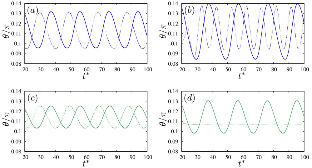
FIGURE 22 – Impact of switching from the quasi-spherical (a,c) to the discocyte (b,d) reference shape on inclination angle in tank-treading regime at \lambda = 0.4 , Ca(\dot{\gamma}, \mu_s) = 0.5 , for capsule (blue) and capsule–capsule (green). The RBC’s axis of symmetry is initially in the shear plane (solid line) or aligned with the axis of vorticity (dotted line).
