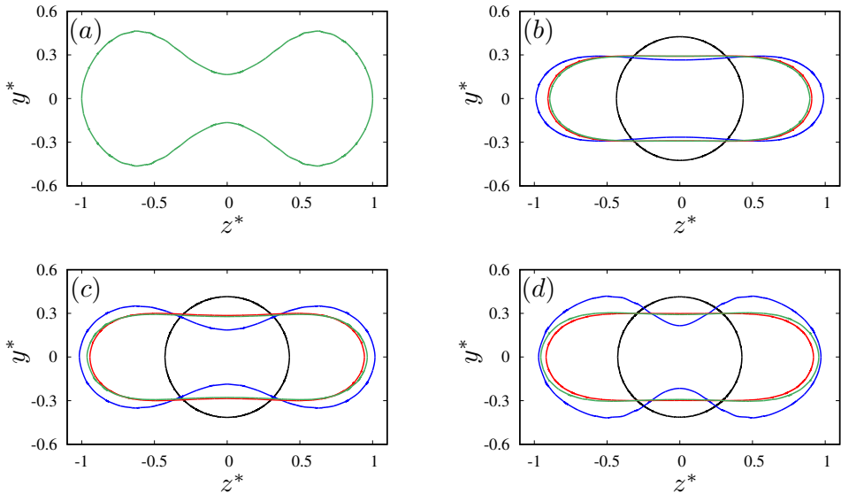
FIGURE 14 – Shape evolutions ( (y^*, z^*) plane sectional drawing) in tank-treading regime at \lambda = 0.4 , Ca(\dot{\gamma}, \mu_s) = 0.5 in the transition phase at t^* = 0 (a), t^* = 6 (b), t^* = 11 (c) and t^* = 15 (d), when the RBC's symmetry axis is in the shear plane at the start (vesicle = black, capsule = blue, vesicle-capsule = red, capsule-capsule = green).
