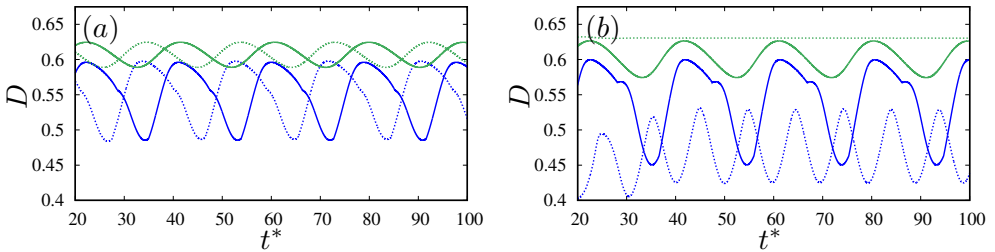
FIGURE 23 – Impact of switching from the quasi-spherical (a) to the discocyte (b) reference shape on deformation in tank-treading regime at \lambda = 0.4 , Ca(\dot{\gamma}, \mu_s) = 0.5 , for capsule (blue) and capsule–capsule (green). The RBC’s axis of symmetry is initially in the shear plane (solid line) or aligned with the axis of vorticity (dotted line).
