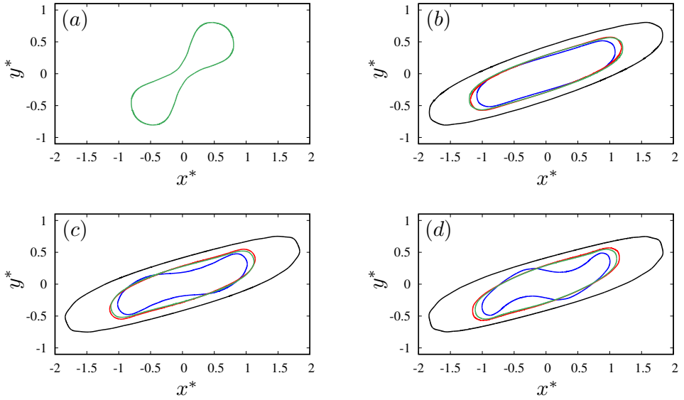
FIGURE 13 – Shape evolutions ( (x^*, y^*) plane sectional drawing) in tank-treading regime at \lambda = 0.4 , Ca(\dot{\gamma}, \mu_s) = 0.5 in the transition phase at t^* = 0 (a), t^* = 6 (b), t^* = 11 (c) and t^* = 15 (d), when the RBC's symmetry axis is in the shear plane at the start (vesicle = black, capsule = blue, vesicle-capsule = red, capsule-capsule = green).
