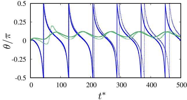
FIGURE 21 – Time evolution of the inclination angle \theta/\pi in the tumbling to tank-treading transition region at \lambda = 0.417 , Ca(\gamma, \mu_s) = 0.113 , for capsule (blue) and capsule–capsule (green), using the quasi-spherical (solid line) and discocyte (dotted line) reference shapes for the cytoskeleton.
