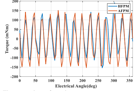
Fig. 17. The comparison of cogging torque
