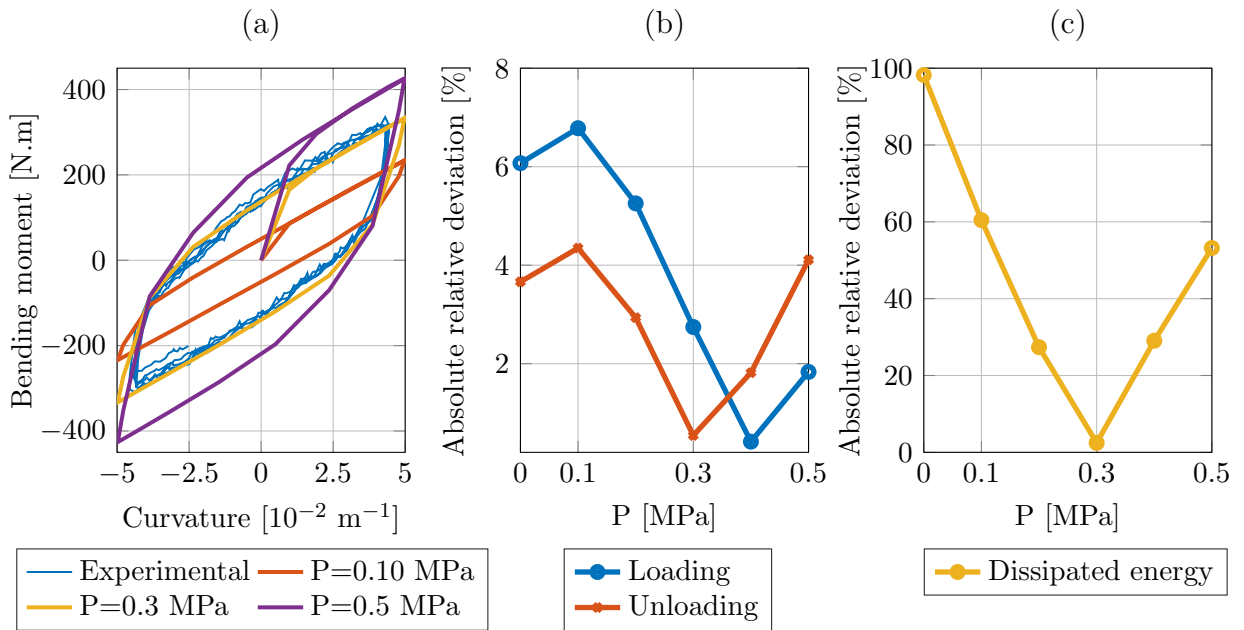
Figure 15: Evolution as a function of the external pressure of: the bending behaviour (a); the absolute relative deviation between the numerical stiffness and the test stiffness at the end of loading and unloading steps (b); the absolute relative deviation between the numerical model and the test in terms of energy dissipated during the bending cycle (c)
