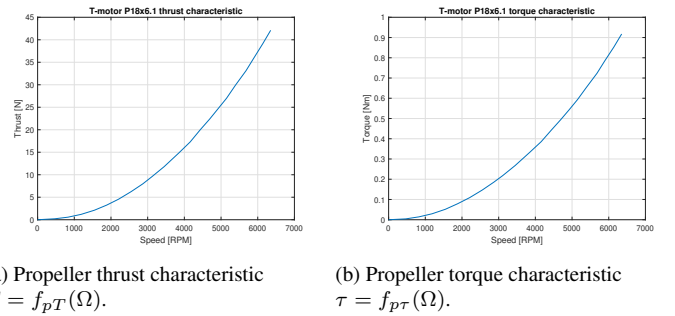
FIG. 6. T-motor P18x6.1 propeller characteristics.
