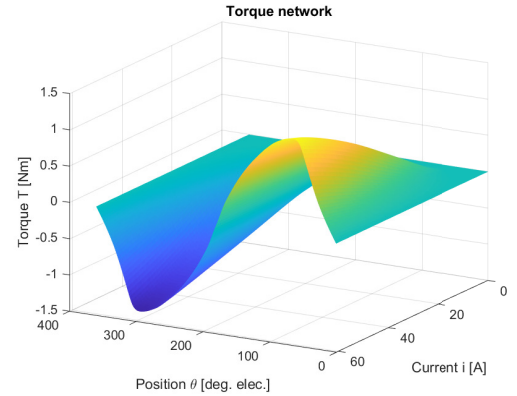
(a) Torque characteristic T = f_t(\theta, i) .
