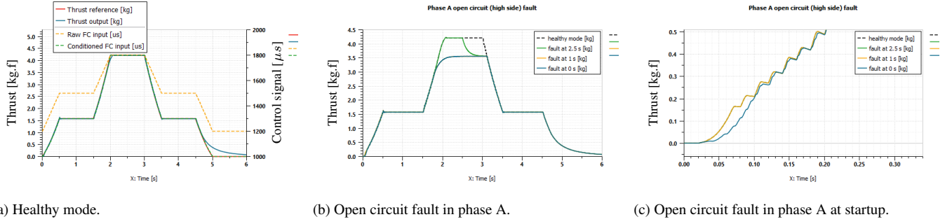
FIG. 4. Switched reluctance motor in a healthy mode and single phase fault operation mode.
