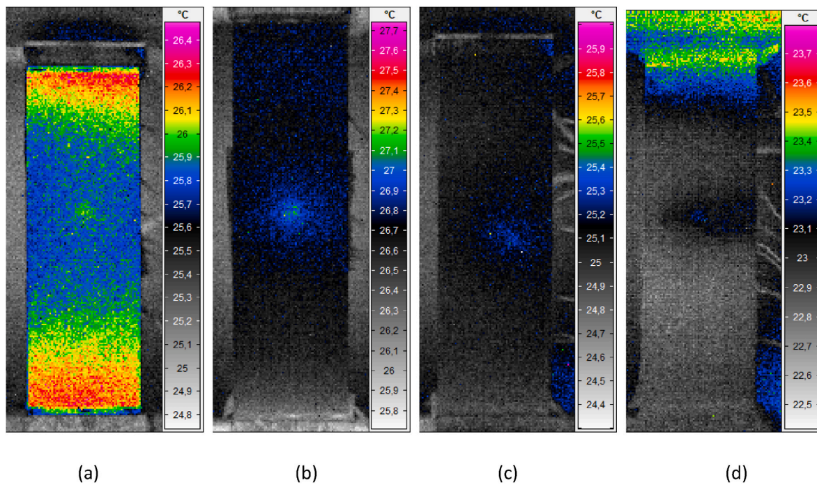
Fig. 13. Exemplary thermograms with detected LVID at the earliest stage for (a) 10J, (b) 20J, (c) 30J, and (d) 40J of impact energy for CFRP specimens.
