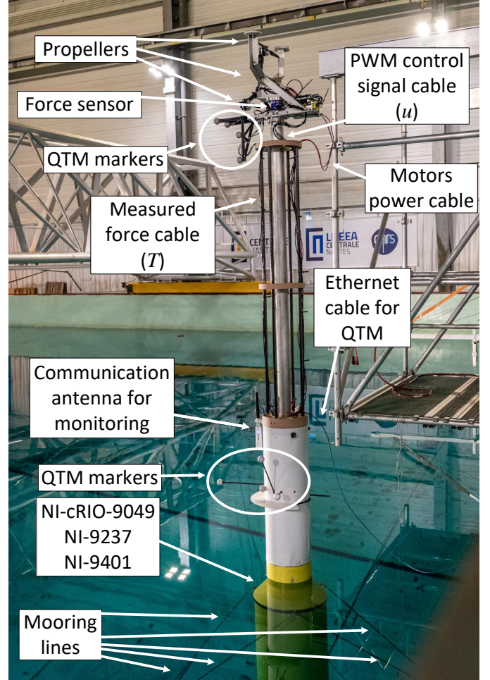
Figure 2: Photograph of the developed reduced-order FWT located in the test tank
