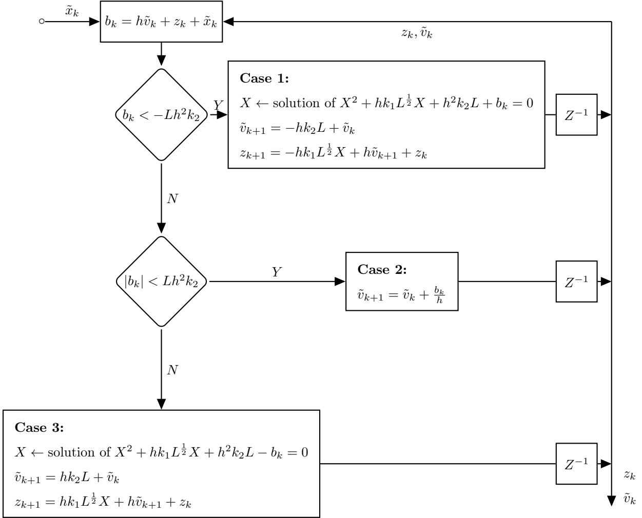
Figure 10: Flowchart of the STD derived from [43]
