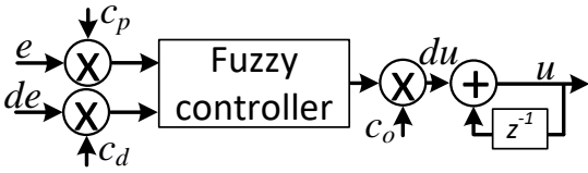
Figure 9: Synthesize the control signal using the fuzzy control block. Note that z^{-1} is the unit delay operator.
