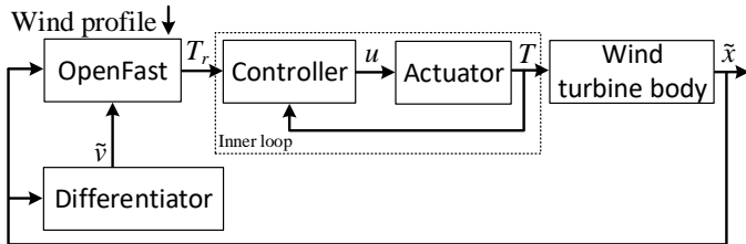
Figure 11: Calculation loops implemented on the computer.
