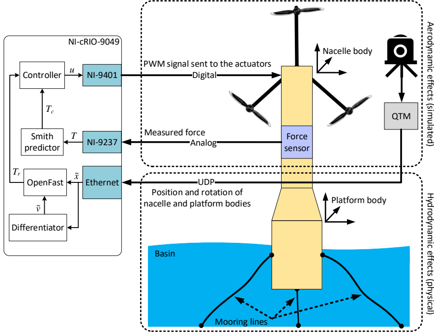
Figure 3: Block diagram of the hardware used for the implementations.
