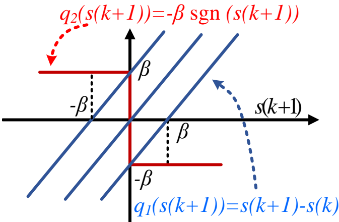
Figure 4: Graphical interpretation of the generalized equation (19), where intersection of these two plots shows the solutions of (19).
