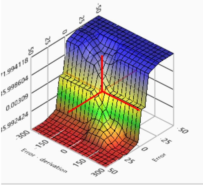
Figure 8: Fuzzy membership functions
