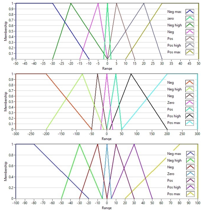
Figure 7: Fuzzy membership functions
