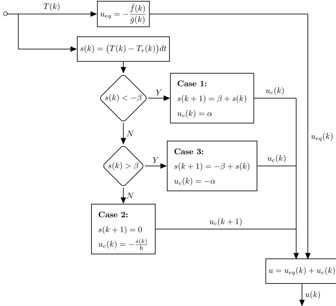
Figure 5: Flowchart of the SMC based on the developed Euler backward discretization. Note that the value of s(k+1) is not used for the next time step in the blocks corresponding to Cases 1 and 3.
