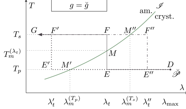
Figure 10: In the plane g = \check{g} , equilibrium curve \mathcal{S} (solid curve), and three cases of paths followed by a crystallite during unload process ( D to G ): \lambda_m^{(T_p)} < \lambda_t < \lambda_m^{(T_s)} (solid arrow), \lambda'_t \leq \lambda_m^{(T_p)} (dotted arrow) and \lambda'_t \geq \lambda_m^{(T_s)} (dash-dotted arrow).
