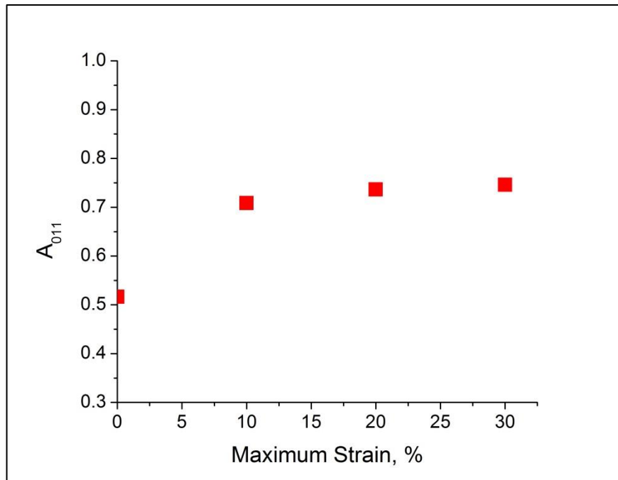
Figure 19. Graph of value of A_{011} against stretch of the nanofibrous membranes.
