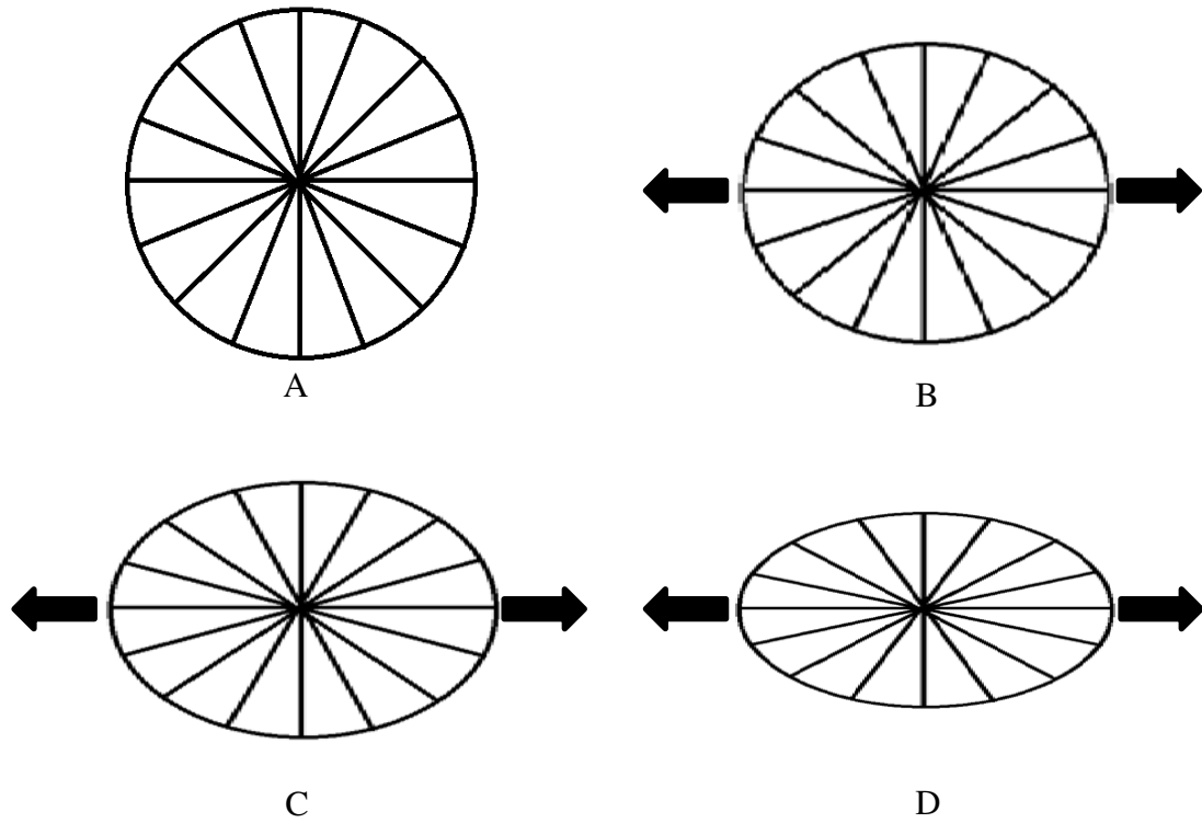
Figure 18. Illustrations of fibers orientation at strain levels A) 0 %, B) 10%, C) 20 % and D) 30 %.
