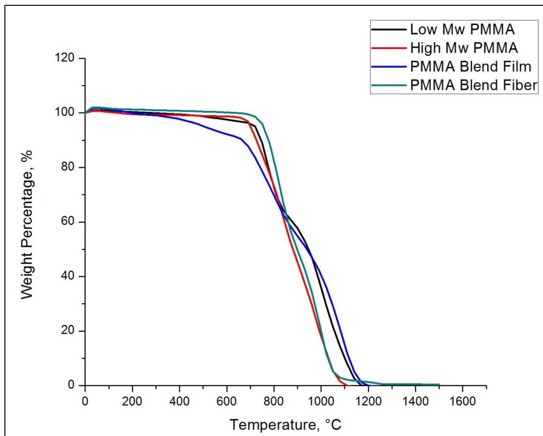
Figure 11. Graph of weight percentage against temperature obtained from TGA.
