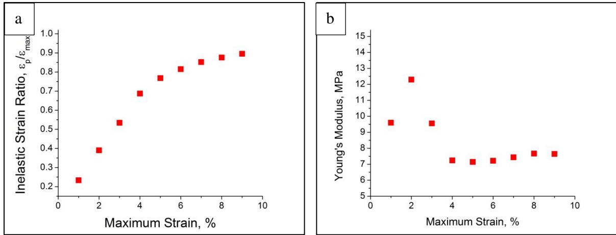
Figure 14. (a) Plot of inelastic strain ratio against maximum strain. (b) Plot of Young's Modulus versus maximum strain.
