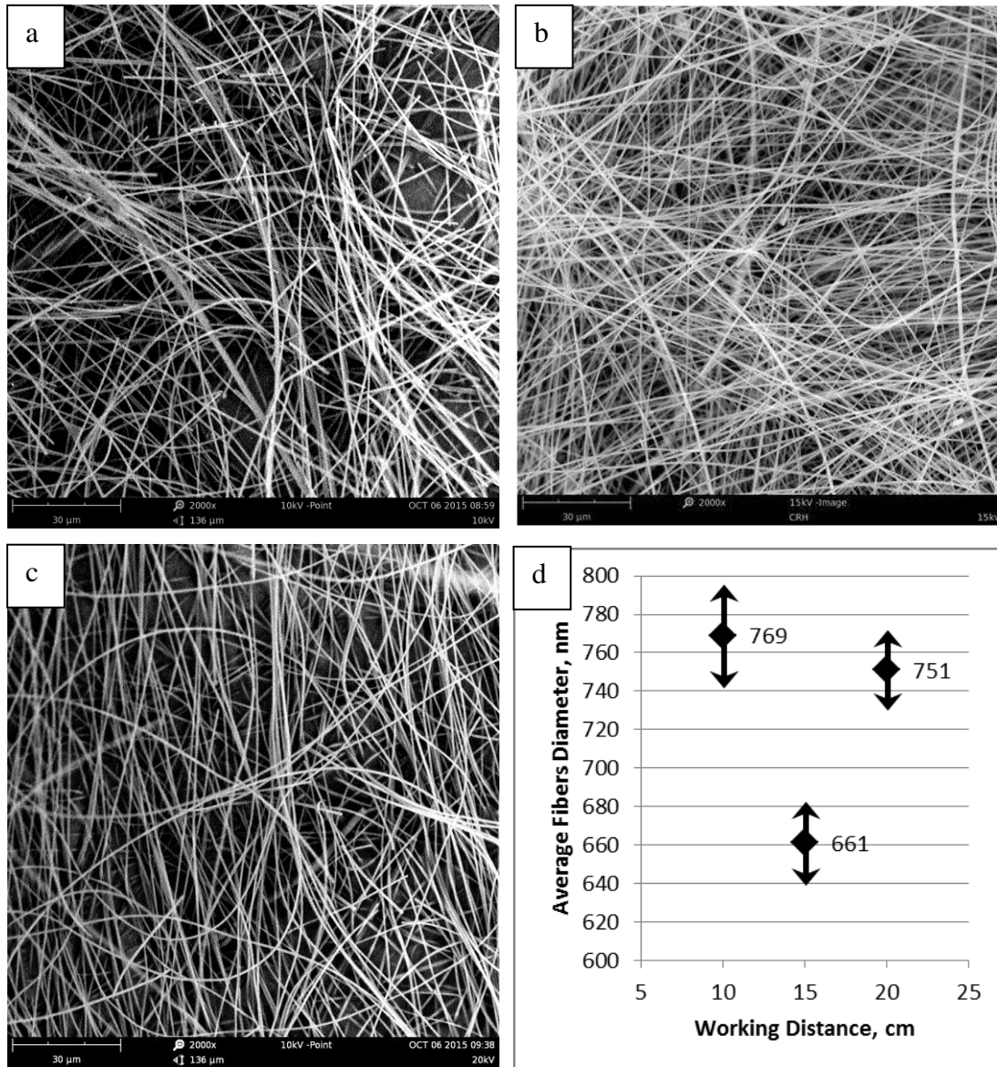
Figure 9. SEM images of Sample (a) D1, (b) F2 (c) D2 and (d) graph of average fibers diameter against working distance.
