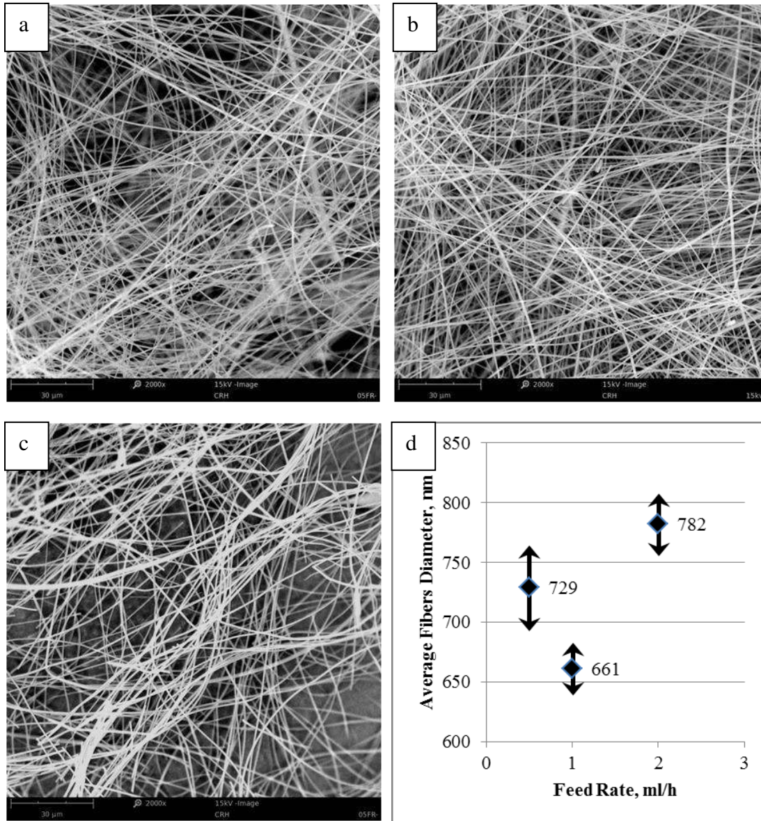
Figure 7. SEM images of Sample (a) F1, (b) F2, (c) F3 and (d) graph of average fiber diameter against feed rate.
