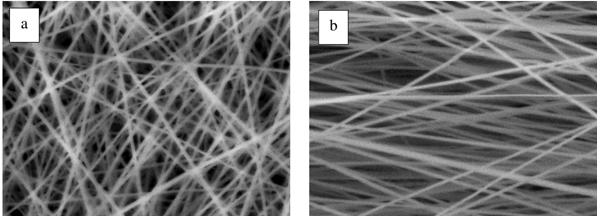
17 Figure 16. SEM images of nanofibrous membrane (a) before being stretched and (b) after 18 being stretched to 30% engineering strain. 19
