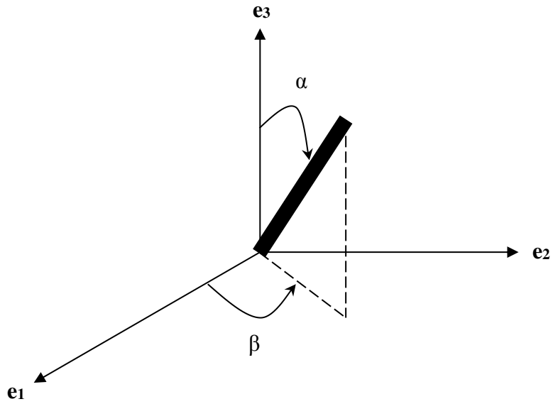
Figure 4. Characterization for an arbitrary unit direction vector \mathbf{p} by means of Eulerian angles in a three-dimensional Cartesian coordinate system.
