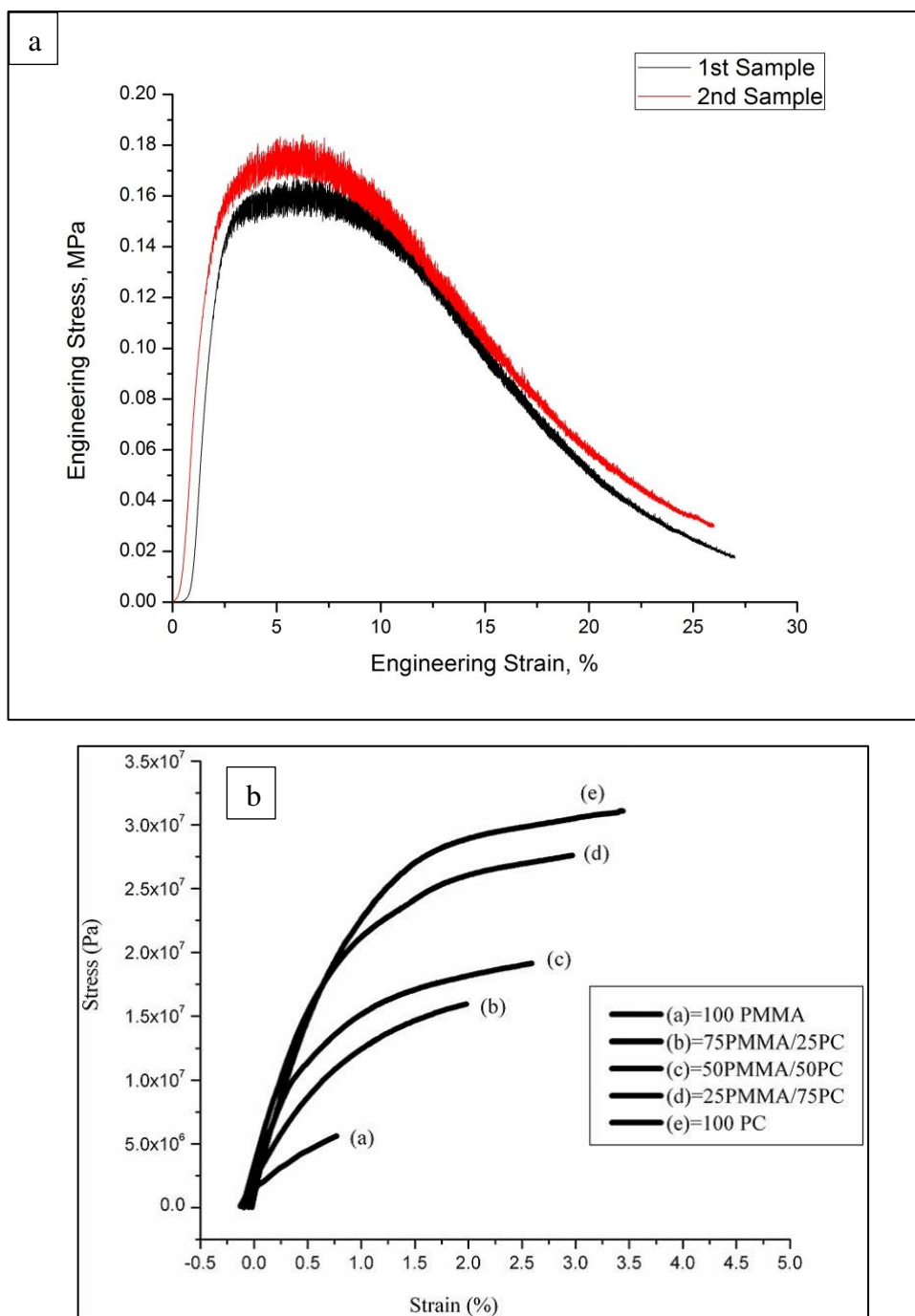
Figure 12. (a) Stress-strain curve of two samples at strain rate of 0.00055 \text{ sec}^{-1} under monotonic tensile, (b) stress-strain curve of PMMA/PC film at different weight ratios [46]
