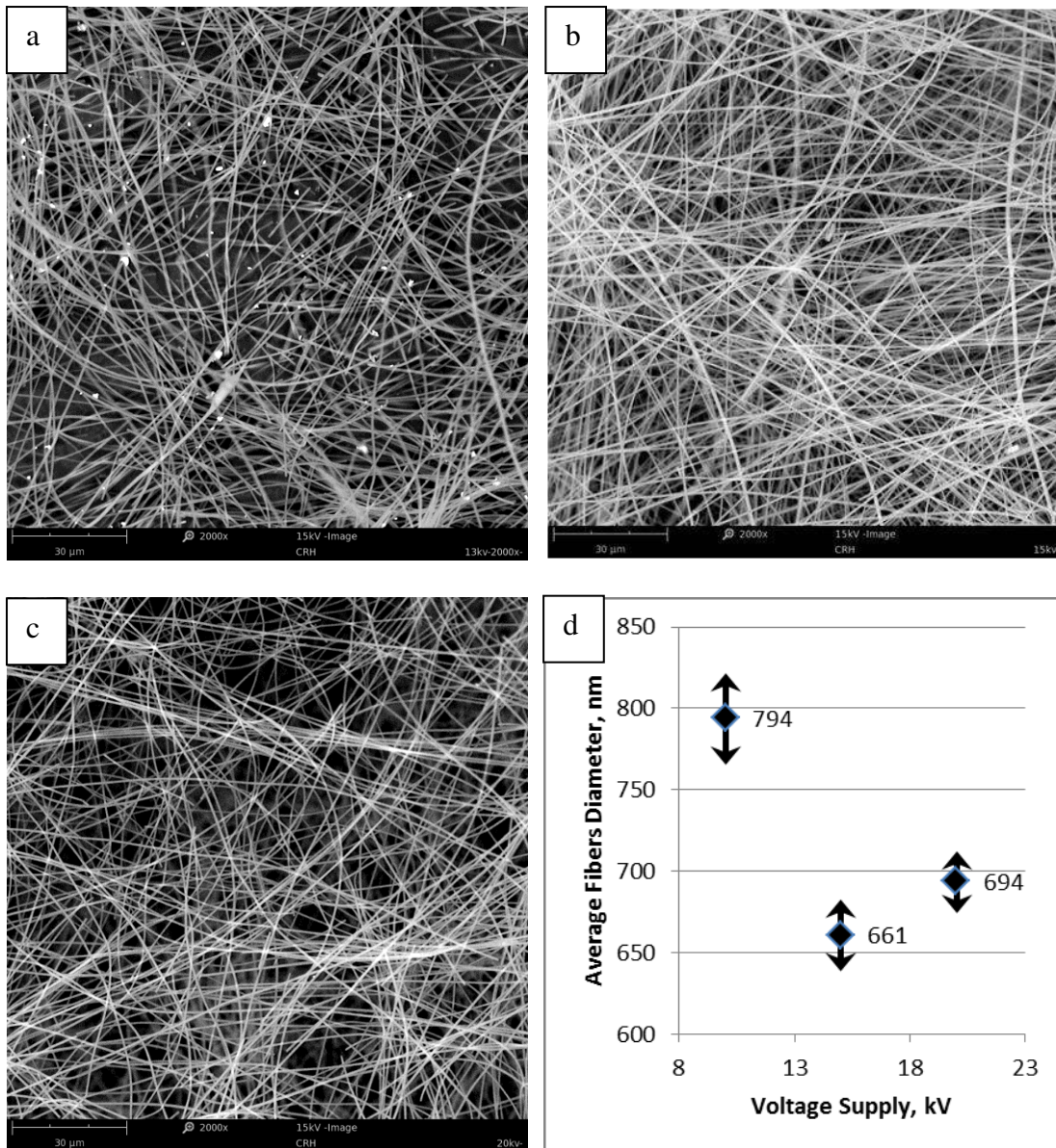
Figure 8. SEM images of Sample (a) V1, (b) F2 (c) V2 and (d) graph of average fibers diameter against supply voltage.
