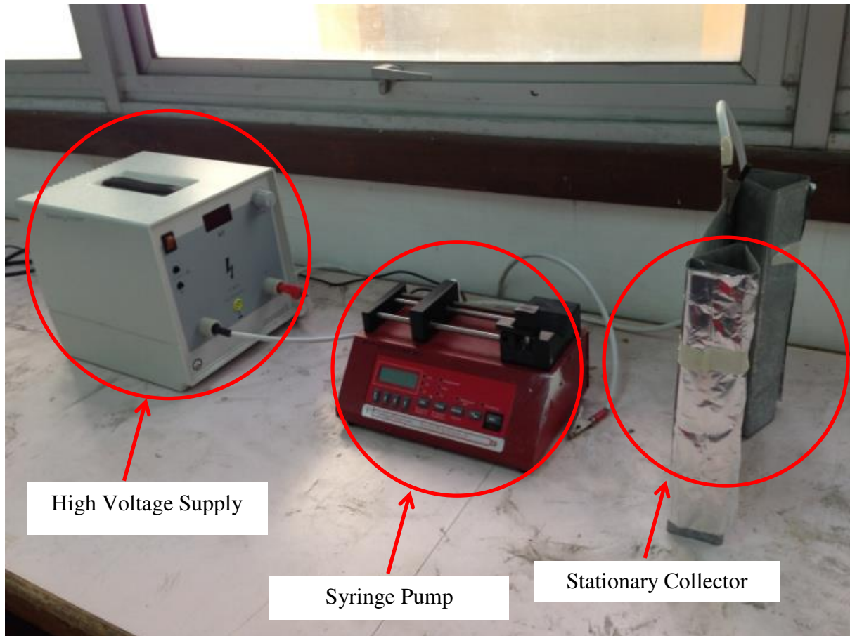
Figure 1. Setup for electrospinning.
