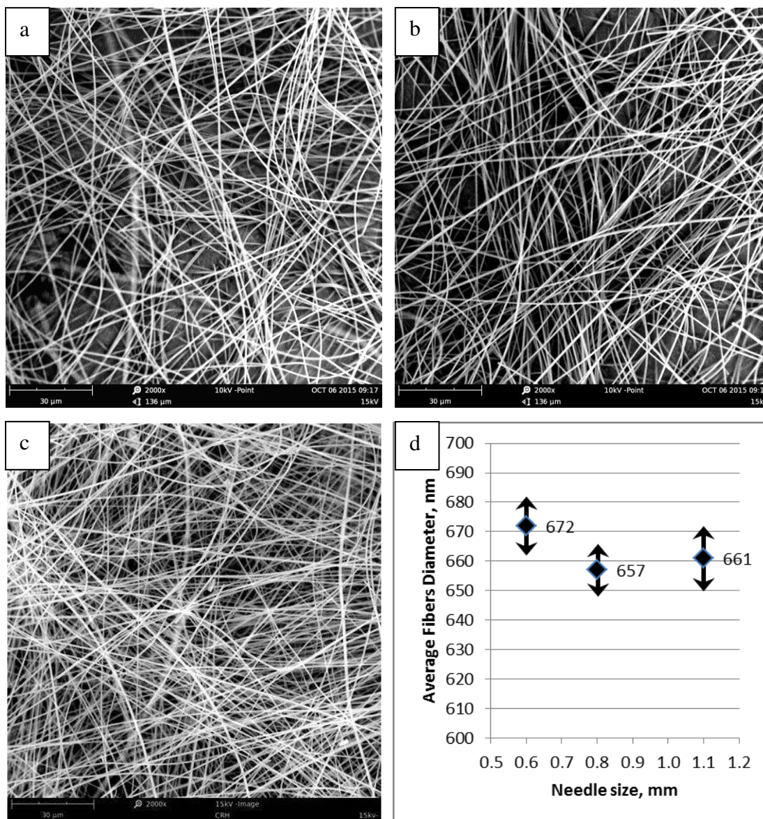
Figure 10. SEM images of Sample (a) G1, (b) G2 (c) F2 and (d) graph of average fibers diameter against gauge size.
