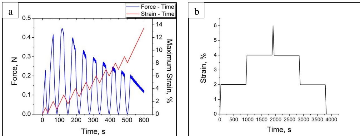
Figure 2. Loading profile for (a) cyclic loading test and (b) cyclic-relaxation test.
