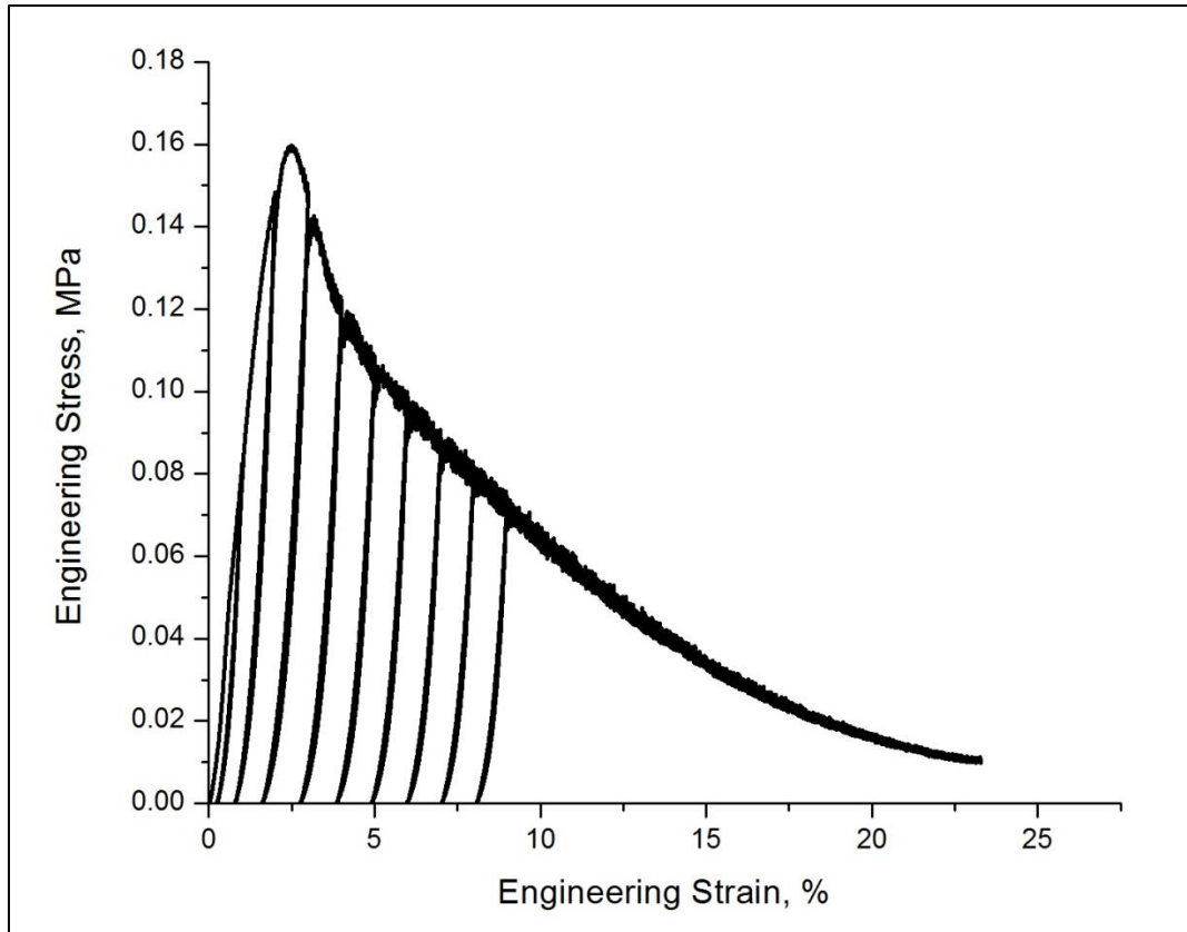
Figure 13. Stress-strain curve obtained from cyclic loading of Sample F2 at strain rate of 5.5 \times 10^{-4} \text{ sec}^{-1} .
