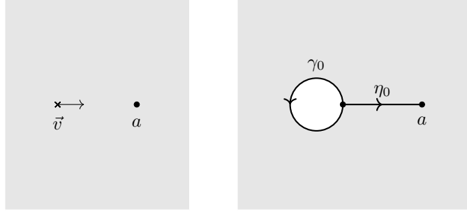
(A) The pair (\mathbb{A}^1 \log \{0\}, \{\vec{v}, a\})
