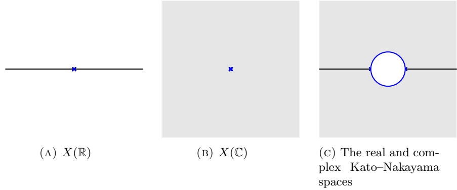
FIGURE 5. Geometry of the log scheme X = \mathbb{A}^1 \log \{0\} , which is defined over any ring \mathbb{K} . The portions of the diagram shown in blue correspond to the log subscheme \partial X = \{0\} \log \{0\} , which gives the boundary of the Kato–Nakayama space.
