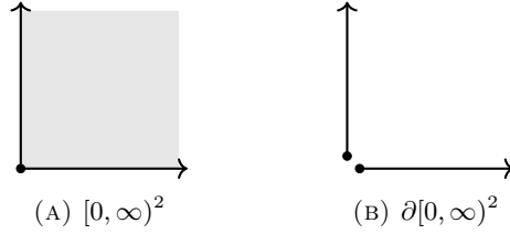
FIGURE 1. The boundary of the quadrant [0, \infty)^2 is the disjoint union of two copies of [0, \infty) .
