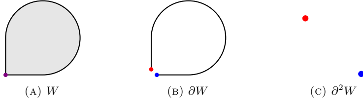
FIGURE 2. The “teardrop” manifold W is a compact surface with a single corner and a single boundary component. Its double boundary consists of two points that are interchanged by the action of \mathfrak{S}_2 , and correspondingly have the same image in W .
