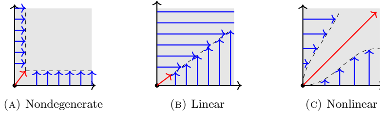
FIGURE 4. Regularizations of the quadrant \Sigma = [0, \infty)^2 , showing the scale on \partial\Sigma in blue, and the scale on \partial^2\Sigma in red.
