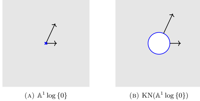
FIGURE 6. Algebraic vs. C^\infty tangential basepoints at the origin in \mathbb{A}^1 .
