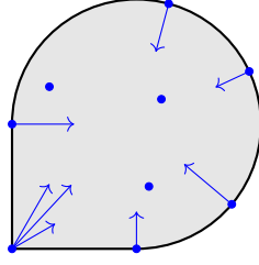
FIGURE 3. Some tangential basepoints on the teardrop manifold.
