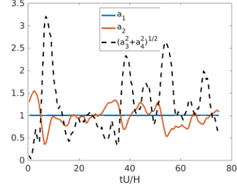
Figure 5. Amplitudes Time evolution of the amplitudes of the POD modes – the deviation mode ( a_2 ) and the intensity of the modes associated with horizontal vortex shedding ( a_3^2+a_4^2 ) 1/2
