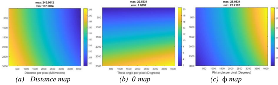
Fig. 6. Distance and angular( \theta, \phi ) per pixel maps.
