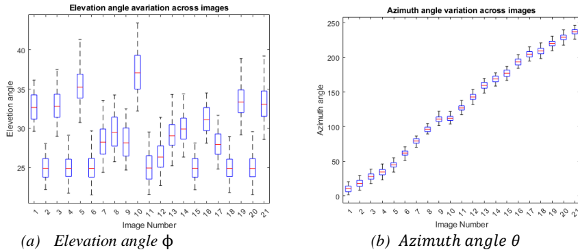
Fig. 7. Angular variation across pixels on first 21 images of the dataset ColorChecker GRAY BALANCE.
