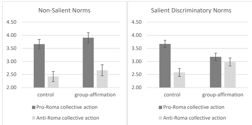
Figure 2. Estimated means and standard errors for collective action as a function of affirmation status and discriminatory norms (Study 2).
