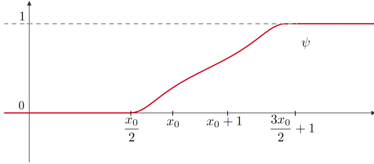
FIG. 2.1. Graph of the function \psi(x) .
