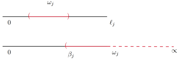
FIG. 0.2. Structure of acted region (in red) in the case of bounded and unbounded branch.
