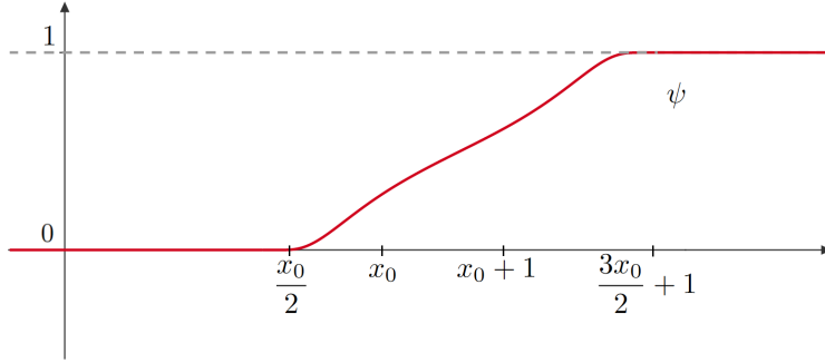
FIG. 2.1. Graph of the function \psi(x) .
