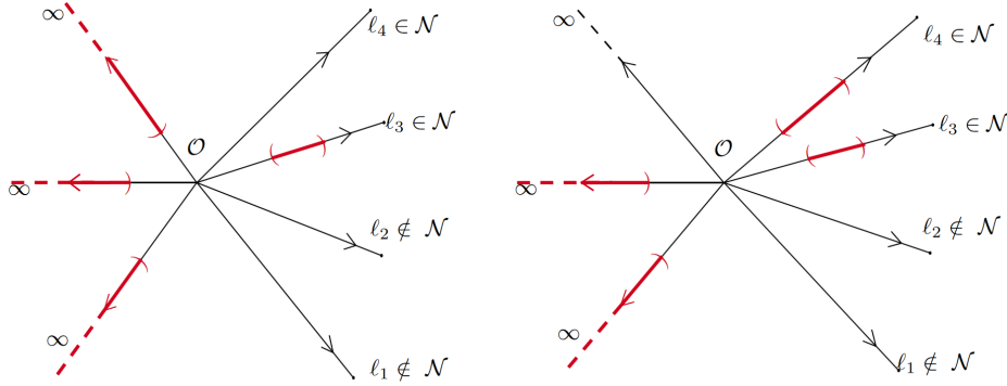
FIG. 3.1. Possible acted branches of Theorem 3.1 and Theorem 3.3
