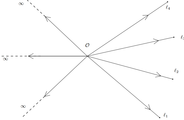
FIG. 0.1. Star shaped network for N_F = 4 and N_\infty = 3 .
