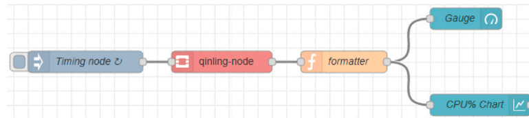
Fig. 9. Node-RED flow involving a Qinling-node.
