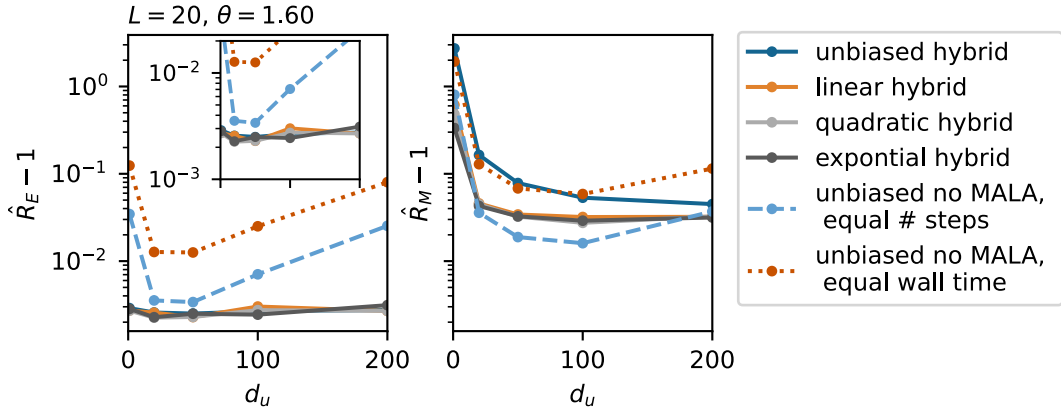
Figure 7: Comparison of the convergence for energy E and magnetisation M for the hybrid (global-local) sampler with biased partial update proposals for different schemes described in the main text. For comparison, we also show results for the simple GlowMC with equal chain length (unbiased no MALA) and the same for such chains shortened to have comparable wall time. The inset of the left panel shows the same data with zoomed-in y-axis.
