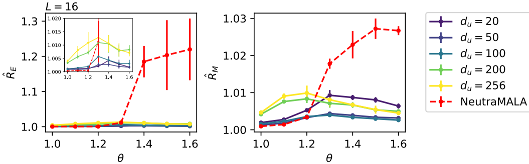
Figure 5: Statistics of GflowMC and NeutraMALA chains at different temperatures \theta . Different update subset sizes d_u are shown for GflowMC. NeutraMALA was run with target acceptances 0.2, 0.5, 0.75, and in each case the best performing strategy is shown. The inset of the left panel shows the same data zoomed in. An average was taken over four independently trained flows, with the standard deviation indicated by error bars.
