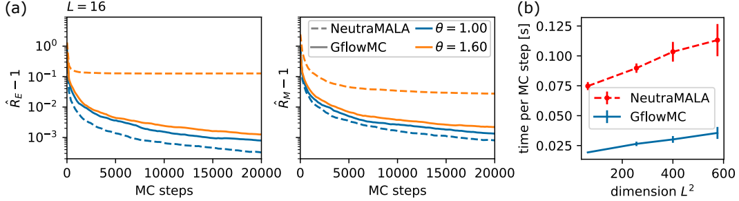
Figure 4: Comparison of samplers utilising a trained normalising flow: NeutraMALA and GflowMC. (a): Convergence of MCMC chains inferred from the observables of energy and magnetisation in the unimodal ( \theta = 1.0 ) and bimodal phase ( \theta = 1.6 ). Both samplers were roughly optimized: For NeutraMALA, the best performing target acceptance out of \{0.2, 0.5, 0.75\} was chosen, for GflowMC, the optimal value of d_u for each observable was chosen, see fig. 3. (b): Wall time per MC step (500 chains evolved in parallel on identical GPU nodes).
