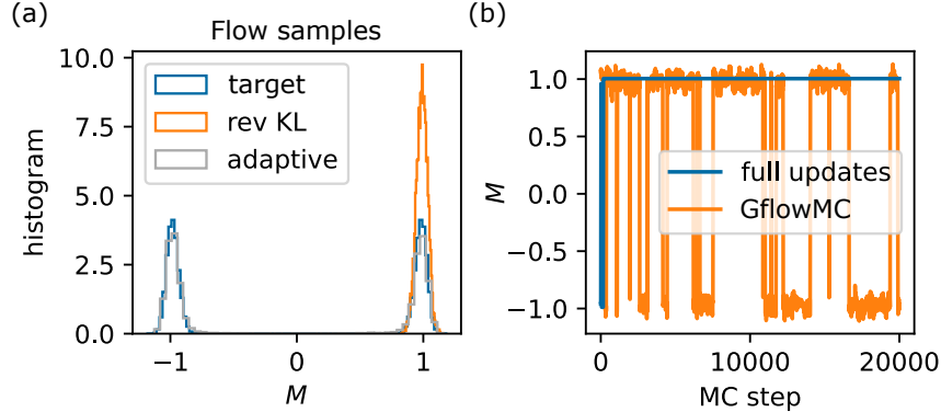
Figure 1: The challenges of using normalizing flows for MCMC sampling of multimodal target distributions in high-dimensions on the example of the 2d \phi^4 model below the critical temperature. (a) Target distribution of magnetisations and samples from two flows trained with the reverse KL divergence as the objective and in the adaptive fashion by (19). The former flow suffers from the well-known mode collapse. The latter flow was used for MCMC sampling in (b). Even when the flow model covers well the two modes, chains with full update proposals suffer from long streaks of rejection and can remain stuck in a single mode. GflowMC chains with partial updates in latent space do not. The plots shown are for L = 20 , and \theta = 1.6 in eq. (4). GflowMC was ran with roughly optimal partial size, d_u = 50 . Out of 500 arbitrarily initialized chains in each case, the worst chain with the least mode switches is shown.
