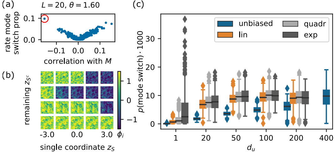
Figure 6: Mode switching abilities of an NF in the \phi^4 bimodal phase, \theta = 1.6 , L = 20 . (a) Mode switching rate for each latent coordinate z_i , determined by how often a mode change is proposed when resampling this coordinate keeping the remaining configuration fixed. (b) Configurations within a row differ by a single latent space coordinate z_S \in \mathbb{R} , chosen by having the largest |c_i| (marked there in red in panel (a)) and varied in [-3, 3] . A single coordinate can induce a mode change in physical space. (c) Mode switching statistics of GflowMC with different update sizes and biasing schemes, chosen to promote the update proposal of coordinates correlated with the mode label.
