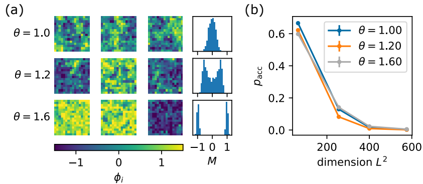
Figure 2: (a) Typical samples and distribution of the magnetisation M of the \phi^4 model at lattice size L = 16 . A phase transition from uni- to bimodal occurs around temperature \theta = 1.2 (35). (b) Using normalizing flows in an IMH sampler (full updates), the acceptance rate quickly vanishes as dimension increases.
