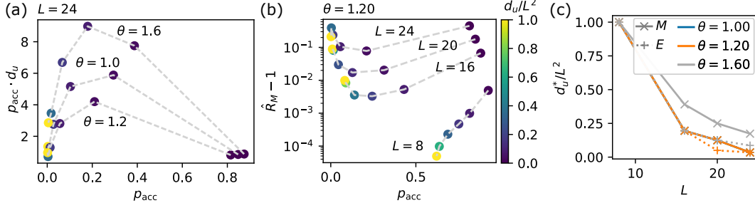
Figure 3: GlowMC convergence as a function of update subset size d_u . (a) Effective update size of chains, and (b) GR statistics for the magnetisation, both shown against the varying acceptance rate. The color indicates d_u/L^2 , the fraction of latent sites for which updates are proposed. For each L , the left-most point with smallest acceptance always corresponds to full updates, the right-most point to single-site updates. (c): Optimal update fraction with increasing lattice size L . Data points in (a) and (b) were obtained as averaged over 4 independently trained flows, and these averages were used to determine each d_u^* in (c).
