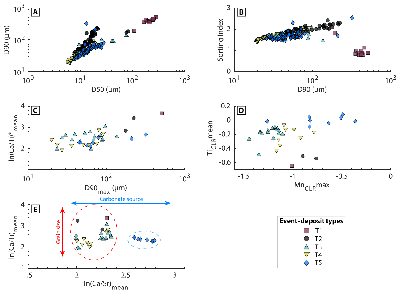
FIGURE 3 Diagrams with selected grain-size parameters and geochemical data for each event-deposit type. (A) D50 versus D90 diagram; (B) D90 versus sorting index diagram; (C) D90 max versus \ln(\text{Ca/Ti})^*_{\text{mean}} diagram; (D) \text{Mn}_{\text{CLR}}^{\text{max}} versus \text{Ti}_{\text{CLR}}^{\text{mean}} ; (E) \ln(\text{Ca/Ti})^*_{\text{mean}} versus \ln(\text{Ca/Sr})_{\text{mean}} diagram. Note that grain-size data are displayed on a logarithmic scale. Diagrams (C–E) display fewer data points because of the different resolutions of the grain-size data (5 mm) and the geochemical data (1–2 mm). “*” denotes that the ratio has been calculated at the depth corresponding to D90 max .
