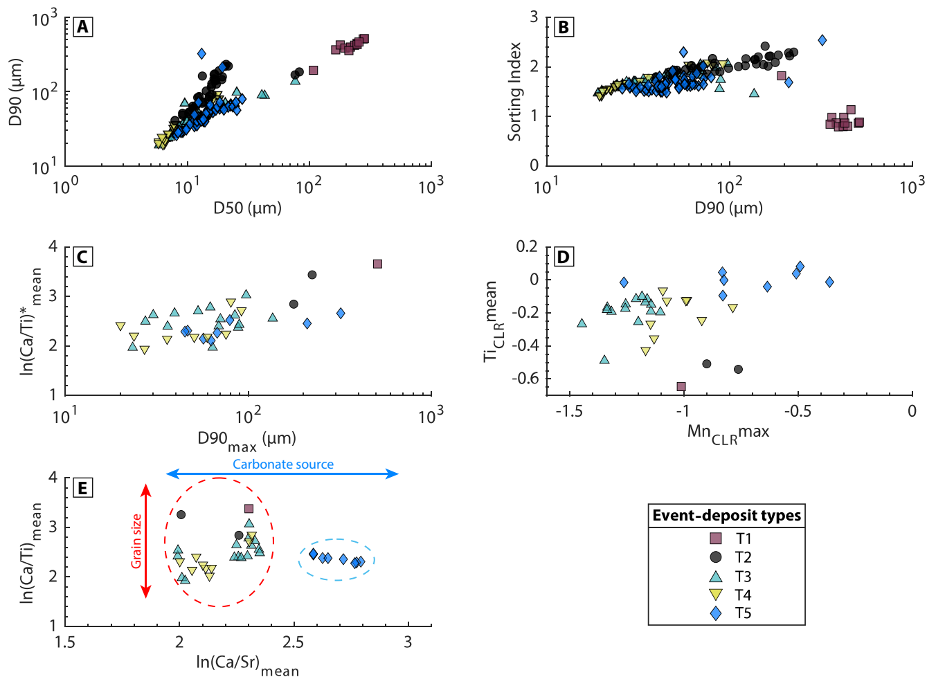
FIGURE 3 Diagrams with selected grain-size parameters and geochemical data for each event-deposit type. (A) D50 versus D90 diagram; (B) D90 versus sorting index diagram; (C) D90_{\text{max}} versus \ln(\text{Ca}/\text{Ti})^*_{\text{mean}} diagram; (D) \text{Mn}_{\text{CLR}}_{\text{max}} versus \text{Ti}_{\text{CLR}}_{\text{mean}} ; (E) \ln(\text{Ca}/\text{Ti})_{\text{mean}} versus \ln(\text{Ca}/\text{Sr})_{\text{mean}} diagram. Note that grain-size data are displayed on a logarithmic scale. Diagrams (C–E) display fewer data points because of the different resolutions of the grain-size data (5 mm) and the geochemical data (1–2 mm). "*" denotes that the ratio has been calculated at the depth corresponding to D90_{\text{max}} .
