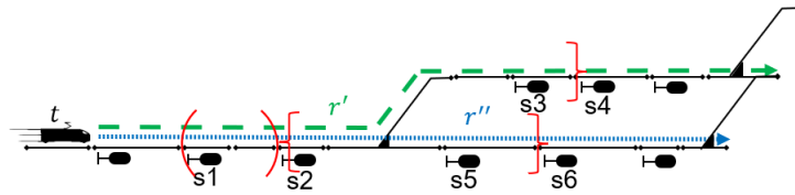
Figure 1 – Graphical representation of relevant sets of block sections: round brackets show set BS' , curly brackets indicate set Ext(\mathcal{R}', BS') for train t having routes r' and r'' available.
