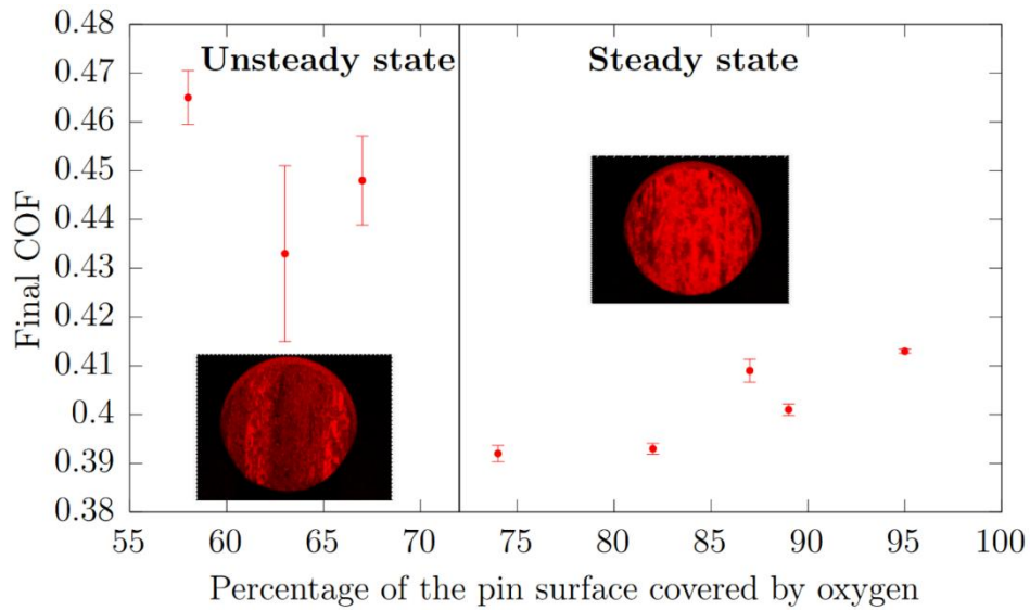
Figure 7. Final COF (average over the last 20 cycles) as a function of the percentage of coverage of the surface of the pin by oxygen (tests performed at 400°C and 600°C and with normal load of F_N = 20 N).
