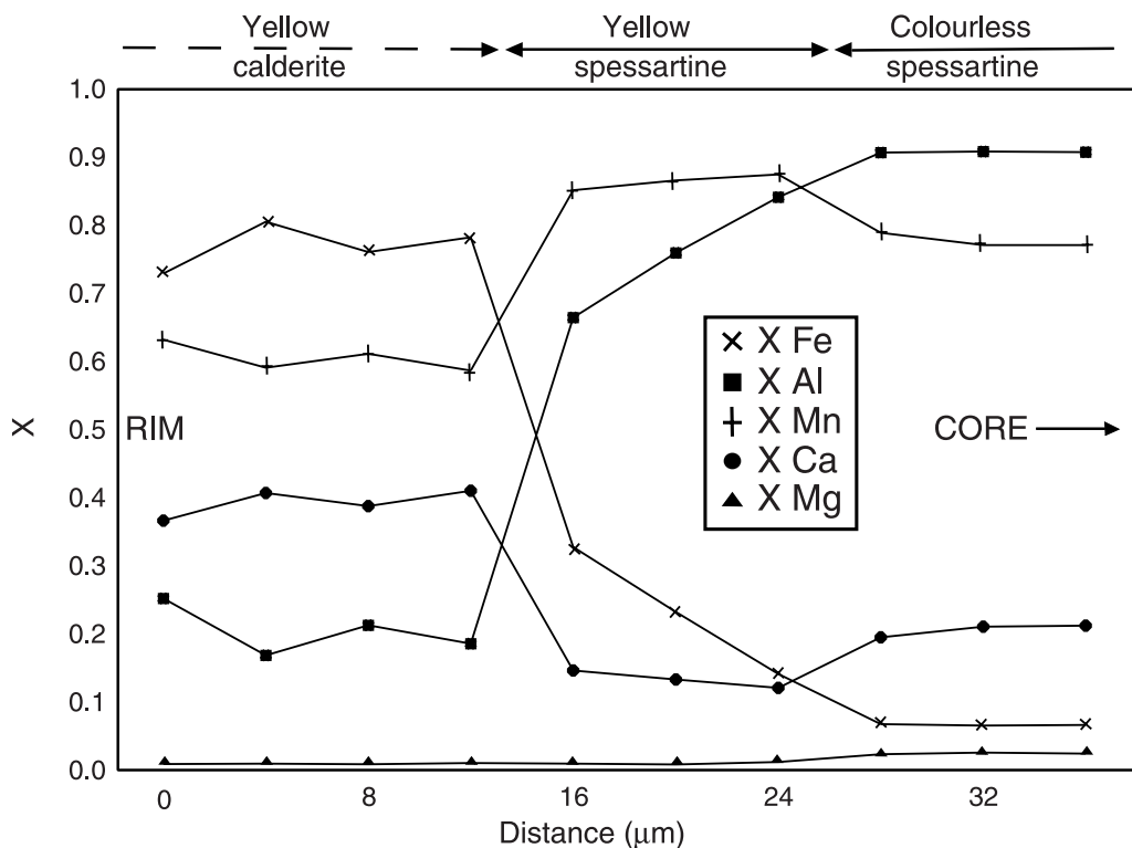
Fig. 6. Analytical traverse (ca. 35 μm) across the contact between spessartine and calderite (#SM-54; see location on Fig. 3d): concentration profiles from EMP analyses. X_{Fe} = Fe / (Fe + Al) ; X_{Al} = Al / (Al + Fe) ; for this figure X_{Mn} = Mn / (Mn + Ca + Mg) ; X_{Ca} = Ca / (Mn + Ca + Mg) ; X_{Mg} = Mg / (Mn + Ca + Mg) . Note the Mn and Ca behaviour in the intermediate zone, which precludes the possibility of mixed analyses
