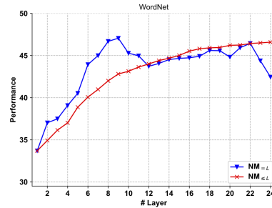
Figure 1: Results of NM =L and NM ≤L per layer for WordNet supersenses with BERT.
