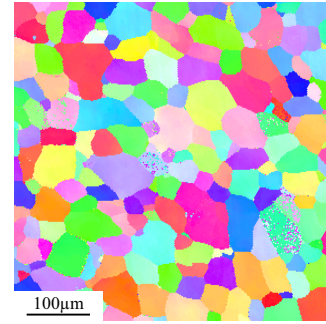
Figure 1: Microstructure of pure iron (ARMCO grade) illustrated by inverse pole figure from electron back-scattered diffraction.
