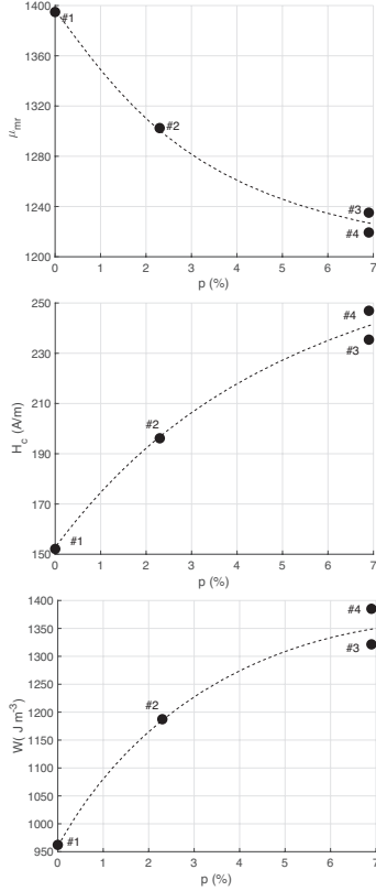
Figure 7: Maximal relative permeability (a), coercive field at H_{max}=8000\text{A/m} (b) and static magnetic energy density losses at B=1.5\text{T} (c) as function of cumulative plastic strain.
