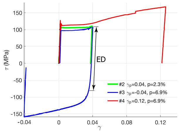
Figure 4: shear stress vs shear strain ( \tau - \gamma ) history of conducted tests. ED: elastic domain after deformation of specimen #2.
