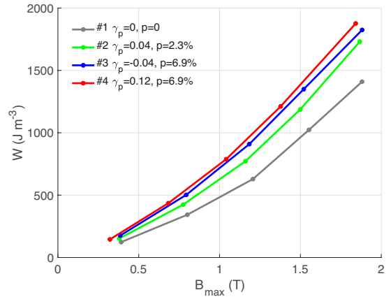
Figure 6: Static magnetic energy density losses for samples #1 to #4
