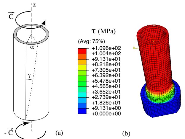
Figure 2: (a) principle of torsion test; (b) optimized (half) geometry and shear stress distribution for C=32\text{Nm} .
