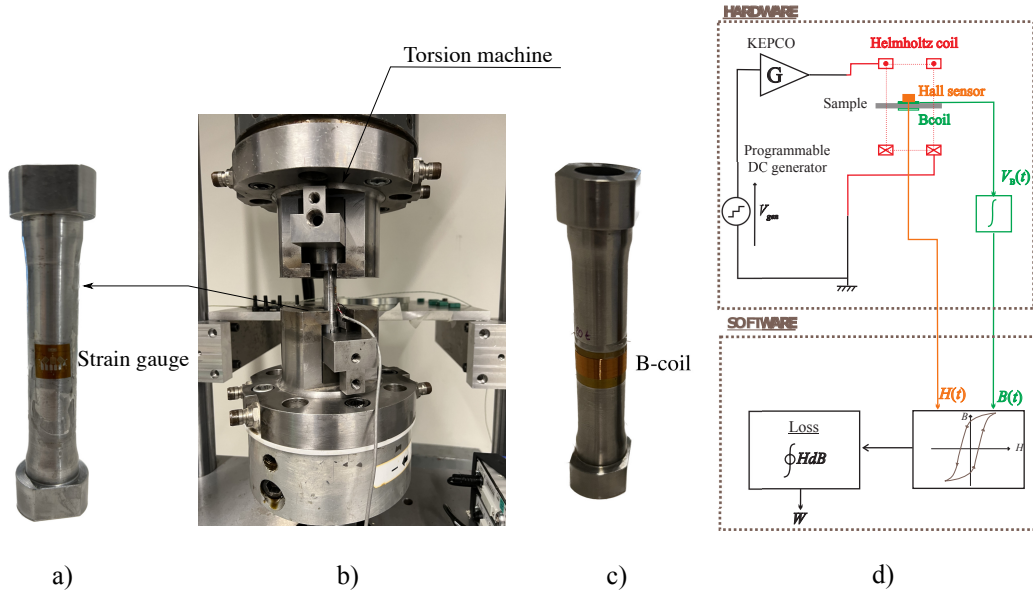
Figure 3: (a) Designed specimen for homogenous shear plasticity ; (b) Testing machine ; (c) specimen after plastic deformation with B-coil; (d) set-up for magnetic measurements
