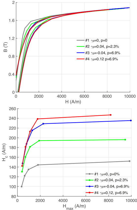
Figure 5: a) Experimental hysteresis cycles for the tested specimens. b) coercive field variation according to maximum magnetic field
