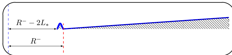
Figure 13: Zoom around the bottomless hole : augmented radial bottom profile (blue line) used for numerical simulations.
