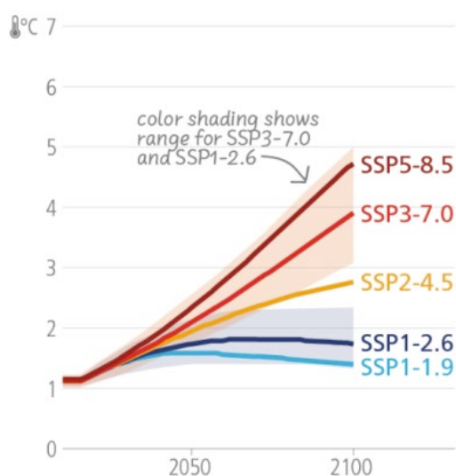
Figure 1 : Temperature for SSP-based scenarios over the XXI th century. © IPCC AR6 SYR Synthesis Report (long report), 2023.
