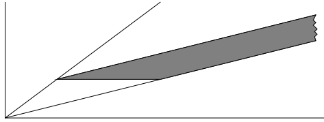
FIGURE 1. The integral of 1/xy over the infinite grey region is finite.
