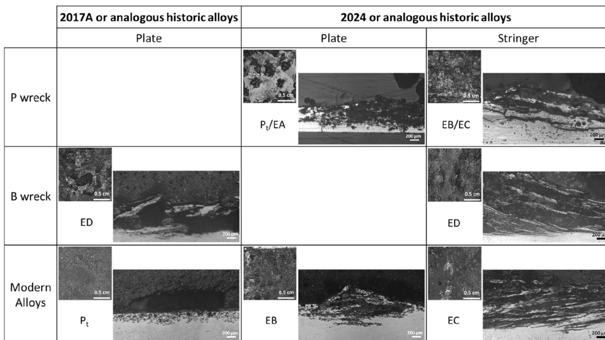
Fig. 8 Optical macrographs of the exposed surface and cross-section images of exfoliated samples after EXCO test (96 h). Under the macrographs is indicated the degree of exfoliation following the classification provided by ASTM G34 ( P_t = pitting; EA = superficial exfoliation; EB = moderate exfoliation; EC = severe exfoliation; ED = very severe exfoliation)
