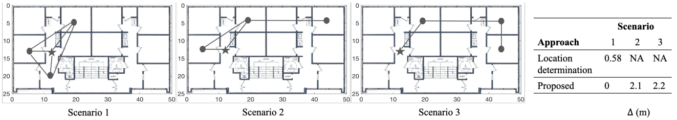
Fig. 12. Comparison with location determination based approach. Star represents the issuer AP, circles represent neighboring APs, and a solid line between two APs means that these are in coverage range of each other. Location determination (Trilateration) based approach can only detect geo-tampering in Scenario 1, where all 4 APs are in each other's coverage range. Our approach is applicable in all three scenarios.
