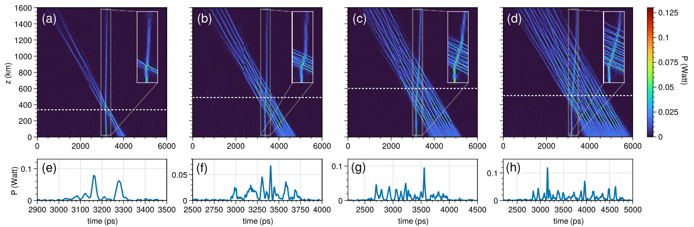
FIG. 2. (a)–(d) Selected set of four space-time diagrams among the 29 available in one single experiment. The shift experienced by the tracer soliton grows with the initial size (duration) of the optical SGs. (e)–(h) Time evolution of the optical power at selected positions (indicated by the horizontal white dashed lines in the top row) where tracer solitons interact with the SGs.
