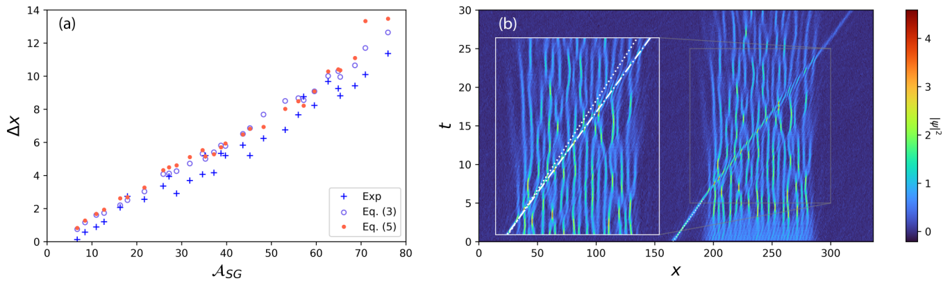
FIG. 3. Comparison between experimental results and theoretical results from the IST theory and the kinetic theory of SG. (a) Shifts measured in the experiment (blue crosses), in numerical simulations of Eq. (3) (empty circles) and using Eq. (5) (solid circles). (b) Space-time diagram showing the interaction between the tracer soliton and the dense SG composed of 24 solitons in the reference frame moving at the group velocity of the SG. The dashed white line following the trajectory of the tracer soliton inside the optical SG has the slope 1/s(\eta_p) \simeq 1/5.26 \simeq 0.19 predicted by the kinetic theory of SGs [Eqs. (6)–(8)].
