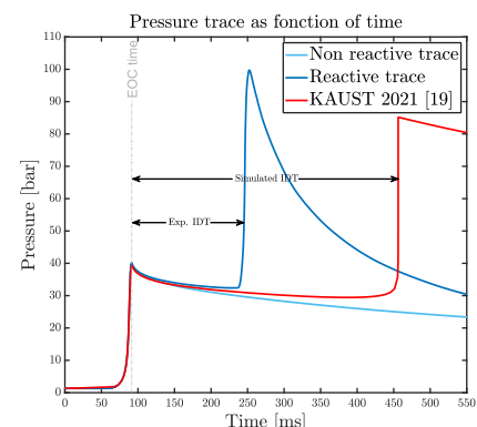
Figure 1: Experimental reactive and non-reactive pressure trace compared with a simulated pressure trace
