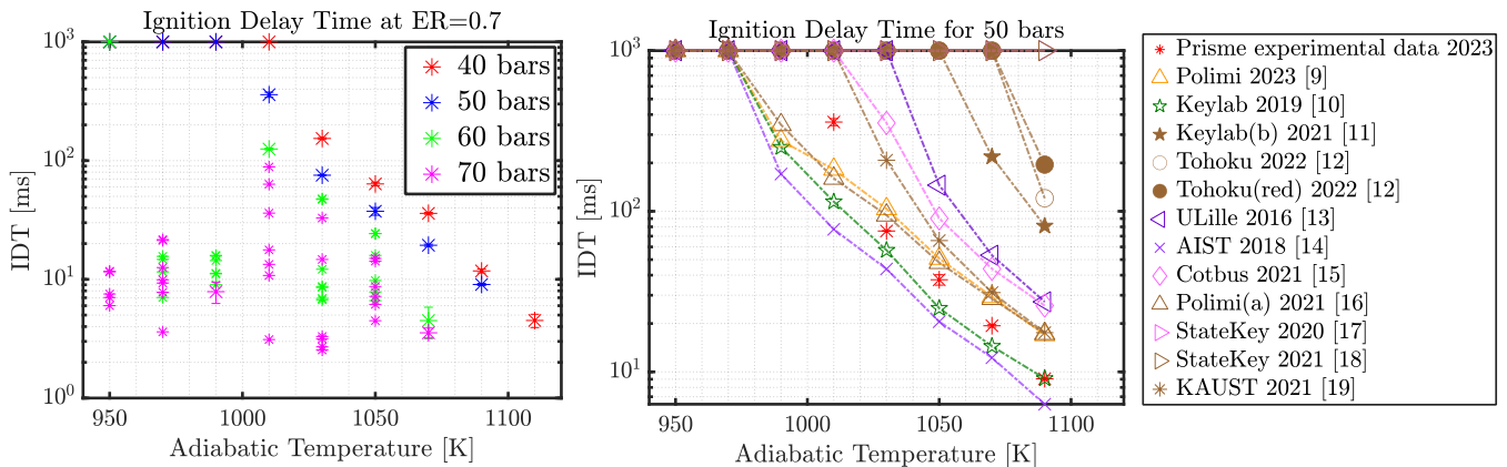
Figure 2: (a-left) Ignition Delay Time at ER=0.7 as function of Temperature for 40 to 70 bars with 10 bars steps. (b- right) Comparison between experimental IDT and simulated IDT from 12 kinetics mechanisms at 50 bars.
