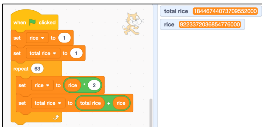
Figure 2. Scratch program with the displayed results to questions 1 and 2
