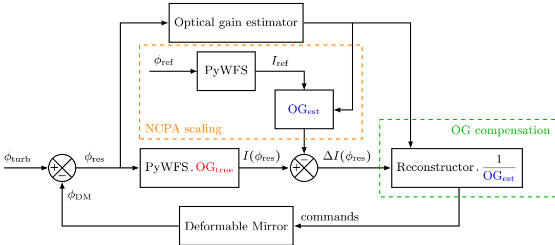
Figure 4. Block diagram of the AO loop representing the action of the optical gains to avoid the NCPA catastrophe and to regain performance.
