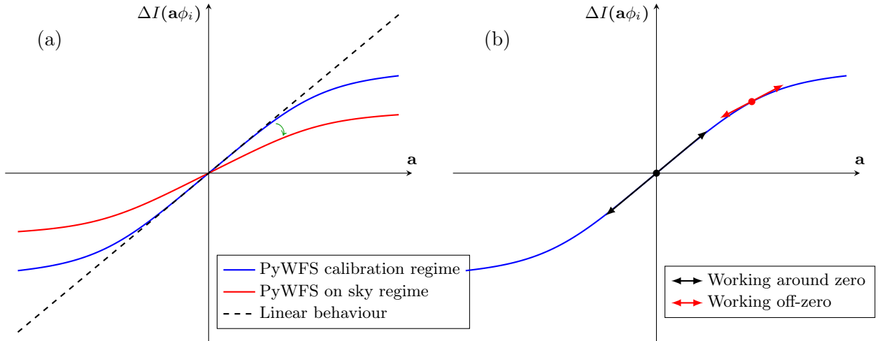
Figure 3. Differential intensity as the output signal of the pyramid for a given mode \phi_i depending on the amplitude a of the mode ; (a) impact of the optical gains on the pyramid signal ; (b) effect of working off-zero.
