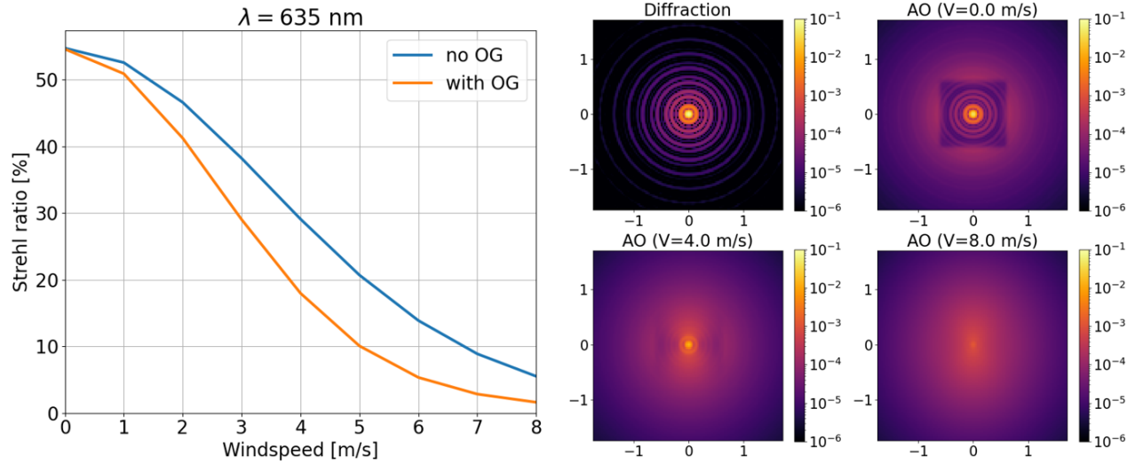
Figure 2. Simulation of Papyrus performances at \lambda = 635 nm with a 2 arcsec seeing conditions and infinite SNR. The four images on the right side show the PSF at diffraction limit (no atmosphere), V = 0 m/s (fitting error only, best performance), V = 4 m/s (moderate wind) and V = 8 m/s (strong wind). X and Y axes of the four PSF images are graduated in arcsec. All the AO computed PSF include the optical gains.
