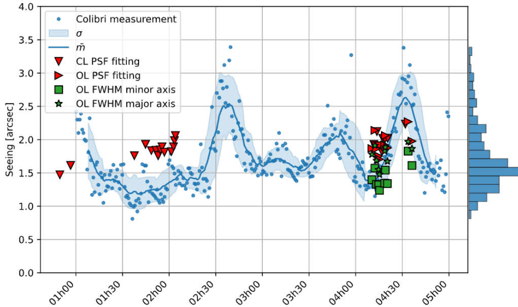
Figure 5. Seeing estimations at OHP on May 26th, 2023. Blue dataset comes from the COLIBRI instrument that was present at OHP at this date, red and green symbols are PAPHYRUS estimations from the PSF image, using PSF fitting and FWHM respectively to estimate the seeing.
