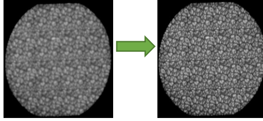
Figure 9. A blurred image due to a turbulence layer at 0km with r_0 ( \lambda 525 nm) of 10 cm (bottom left) and a wide FoV corrected image closing the loop with GLAO.
