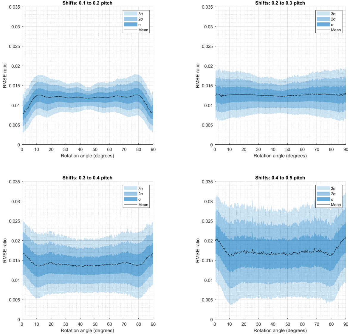
Figure 3-7: Rotation angle against \text{RMSE}_{\text{ratio}} for random linear shifts in the range 0.1 to 0.2 actuator pitch (top left), 0.2 to 0.3 (top right), 0.3 to 0.4 (bottom left) and 0.4 to 0.5 (bottom right). P-Zernike modes cropped at 50, random f^{-2} spectrum incoming phases.
